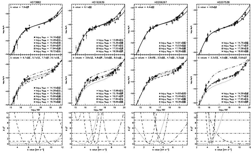
FIG. 1.—COG analysis for \text{H}_2 along the HD 73882, HD 192639, HD 206267, and HD 207538 lines of sight. The top panels assume a common b -value for all J levels. In the middle panels, each J level is fitted with a different b -value. The bottom panels present \Delta\chi^2 as a function of b for the COGs displayed in the middle panels. In the \Delta\chi^2 plots, the different rotational levels are represented by dotted ( J=2 ), dashed ( J=3 ), dot-dashed ( J=4 ), and double-dot-dashed ( J=5 ) lines. Note that due to the nonlinearity of the COG, the \Delta\chi^2 sometimes shows two minima. In these cases, the second minimum is ruled out on the grounds that the resulting column densities are not physical.
