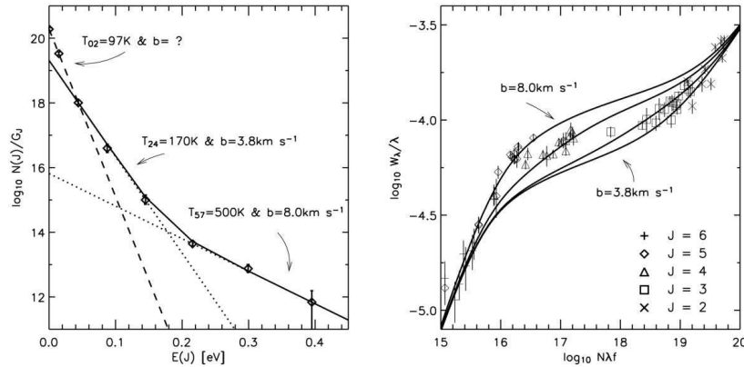
FIG. 5.—Left: Excitation diagram of the \text{H}_2 along the HD 192639 line of sight. We fitted the column densities with several components, with different excitation temperatures and velocity dispersions. The T_{ex} = T_{J-2,4} component is supposed to have a broadening equal to the J=2 species, and the T_{ex} = T_{J-5,7} component a broadening equal to the J=5 species. Right: Two-component COG for J=2-6 , with a relative strength in accordance with the two components fitted on the higher levels of the excitation plot. A variation of the b -values appears due to the presence of the two components.
