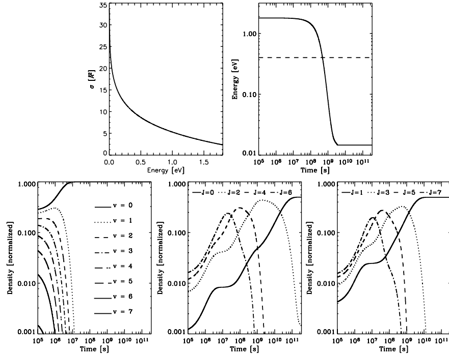
FIG. 7.—Time-dependent model of molecular hydrogen following formation on grains (see the Appendix). Top left : Effective H-H 2 cross section as a function of the kinetic energy. Top right : Kinetic energy of the H 2 molecule as a function of time. The dashed line corresponds to the energy threshold from which C + can react with H 2 to form CH + . Three lower panels : Distribution of H 2 molecules over the vibrational and the ortho and para rotational states, as a function of the molecule's lifetime. Note that radiative vibrational transitions ensure decay toward the vibrational ground state on short timescales. The initial rise of the rotational density curves is due to the cascading of molecules down from the higher J and V levels, whereas the steep drops occur at the radiative lifetime of the level. Because collisional excitation and de-excitation are part of our simulation, all of these plots depend on the density, here equal to 10 \text{ cm}^{-3} .
