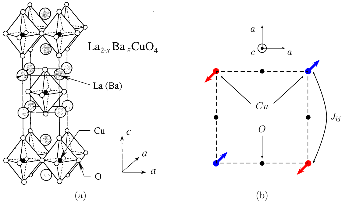
Figure 3.1: (a) Cristallographic structure of the cuprate superconductor La_{2-x}Ba_xCuO_4 and (b) a CuO_2 layer showing the (super)exchange coupling between the copper atoms.
