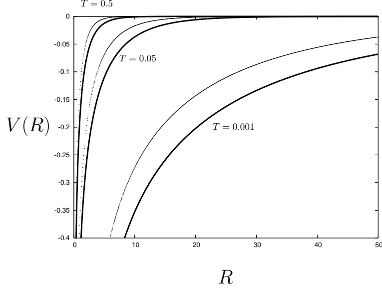
Figure 6.3: Effective static potential with (fat line) and without (dotted line) the Popov-Fedotov imaginary chemical potential for the temperature T = \{0.001, 0.05, 0.5\} .
