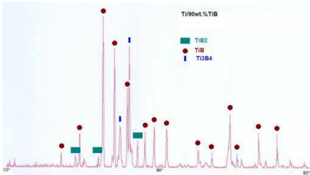
Figure 34: X-ray diffraction pattern for a Ti/90wt.% TiB composition.
