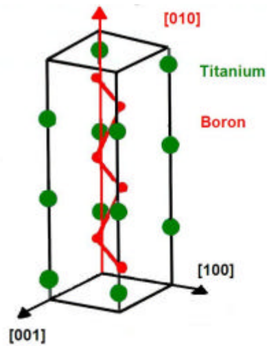
Figure 38: TiB crystal structure (B.F. Decker et al., 1954).
