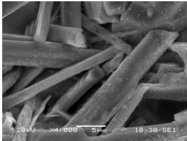
Figure 36: SEM image of the morphology of TiB in the Ti/60wt.%TiB material.
