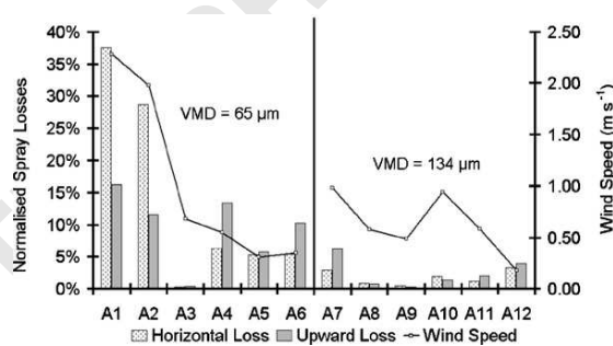
Fig. 4. Normalised spray losses and wind speed for the 12 test of A series.
