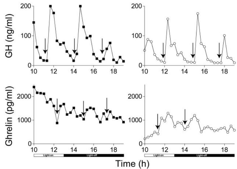
FIG. 5. Representative GH and ghrelin secretory patterns during a 9-h sampling period in two freely moving male rats. Arrows indicate the occurrence of peaks as defined by cluster analysis.
