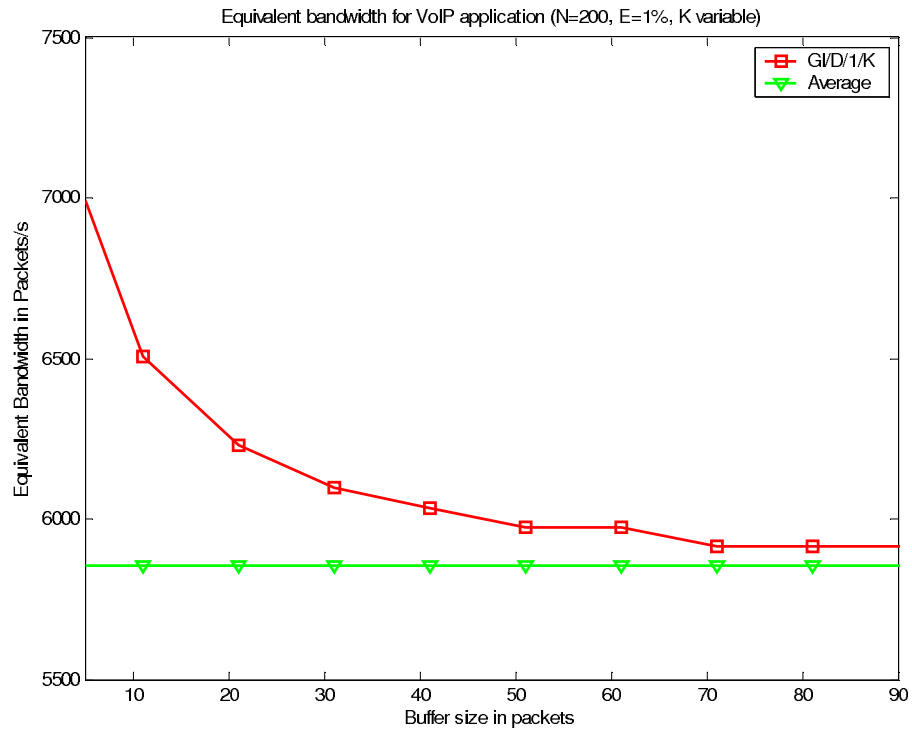
Figure 7.6: G711C Equivalent Bandwidth Estimation (Variable Buffer Size)
