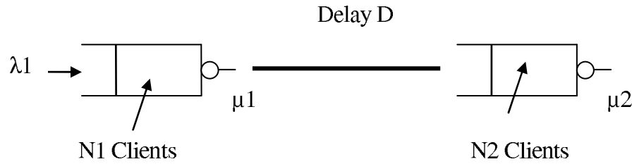
Figure 6.4: Propagation Rules
