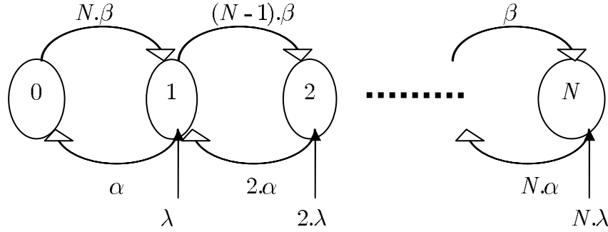
Figure 5.13: MMPP-N+1 Process
