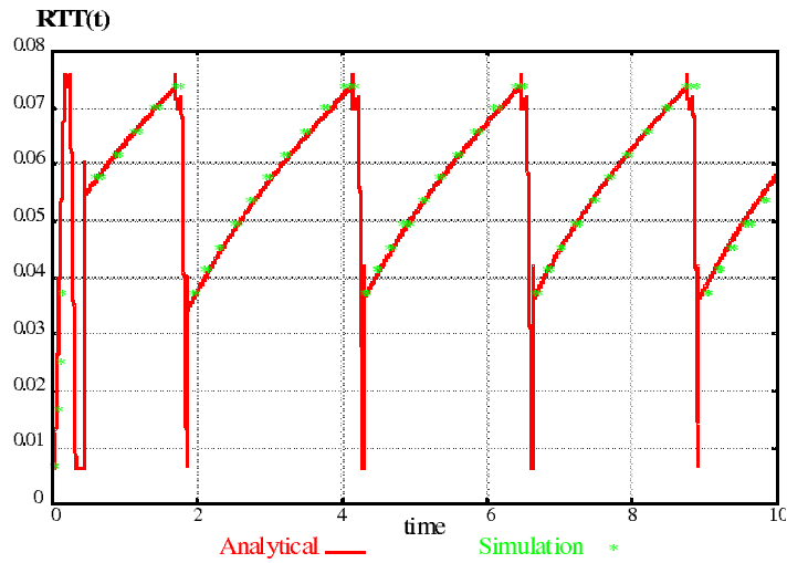
Figure 6.10: RTT Evolution
