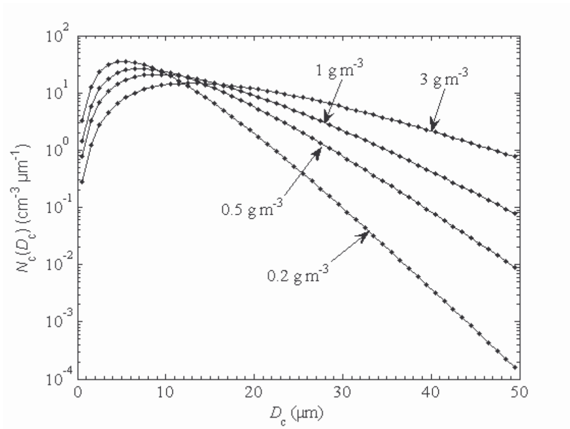
Figure 2: Cloud droplet size distribution (CSD) represented by (7), D_c being the droplet diameter and N_c the volumic concentration per class of diameter. CSD is displayed for four values of M_c^{\max} ( 0.2, 0.5, 1, \text{ and } 3 \text{ g m}^{-3} ) and N_t equal to 350 \text{ cm}^{-3} .
