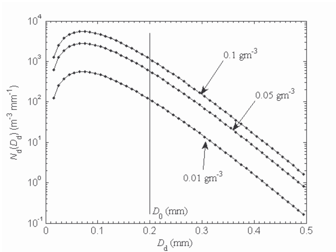
Figure 6: Drizzle drop size distribution (DDSD) for a parameter \mu equal to 2 and several maximum drizzle water content (0.01, 0.05, and 0.1 \text{ g m}^{-3} ). Median diameter is D_0 = 0.2 \text{ mm} (solid vertical line).
