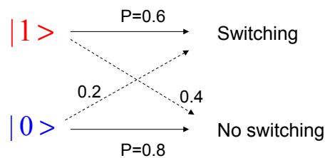
Figure 2.20: Phenomenological model for the readout process. The readout junction has a probability 0.6 to switch if the qubit is in state 1 and a probability 0.2 to switch if the qubit is in state 0.
