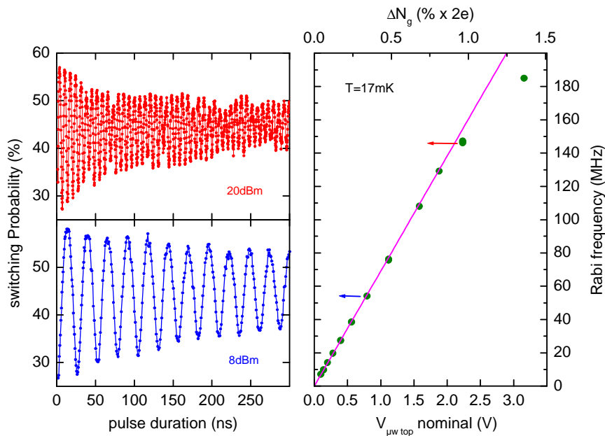
Figure 1.10: Left: Rabi oscillations for 2 different microwave powers. The probability of being in state |1\rangle oscillates with the microwave pulse duration. Right: as expected the Rabi frequency is proportional to the microwave amplitude.
