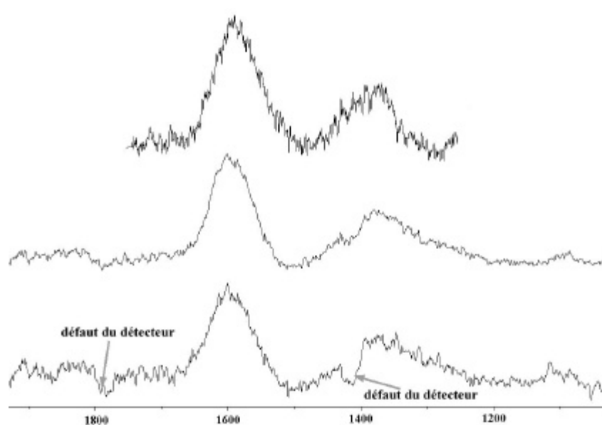
Spectre(s) Raman {17}.
