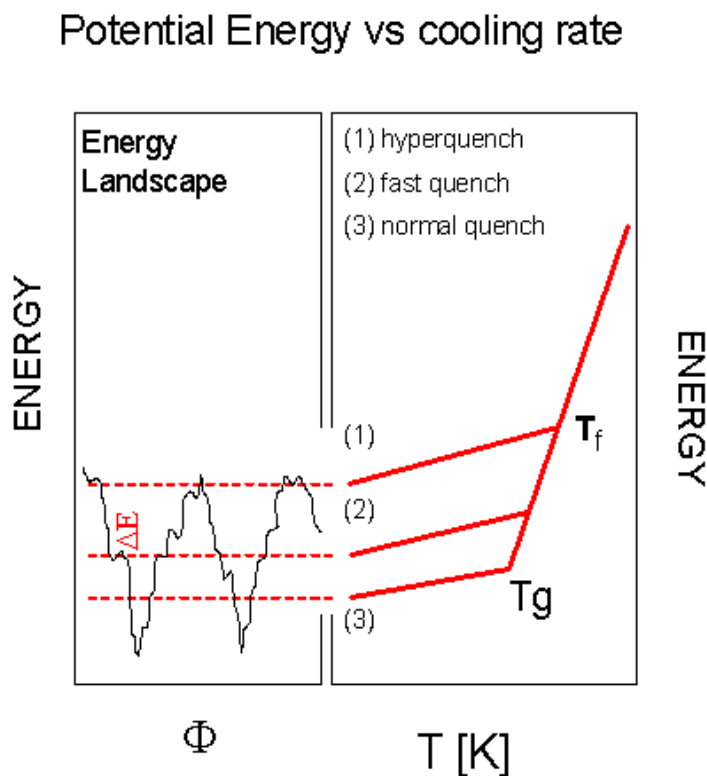
Figure 3.2: Sketch of the energy landscape of a glass (left panel) corresponding to different cooling processes (right panel). \Phi is the coordinate of the space of configurations of the system \Phi = \Phi(r_1, \dots, r_{3N}) .
