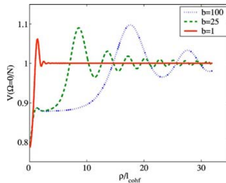
FIG. 10. Squeezing spectrum normalized to the shot noise at zero frequency, and at resonance, as a function of the distance between the two pixels \rho (scaled to the coherence area l_{coh f} ), in the finite pump regime and far-field approach and for different values of b .
