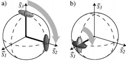
FIG. 13. Visualization of measured quantum noise and measured Stokes vectors of four polarization states mapped onto the Poincaré sphere. The states were generated from (a) two bright amplitude squeezed inputs and (b) a bright coherent beam and an amplitude squeezed vacuum. The rotation in (a) and also in (b) was achieved by a \theta = \pi/2 phase shift or an additionally introduced \lambda/4 wave plate.
