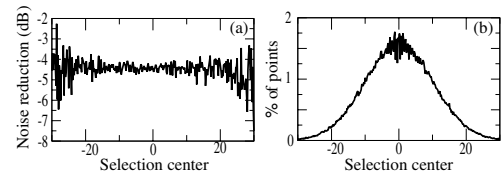
FIG. 5. Measured intensity noise on the reduced state (a) and preparation probability (b) as a function of the band center normalized to \sigma_0 . The selection bandwidth is taken equal to 0.4 times the shot noise.
