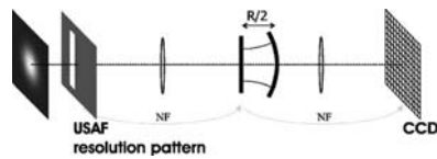
FIG. 9. Schematic representation of the experimental setup.
