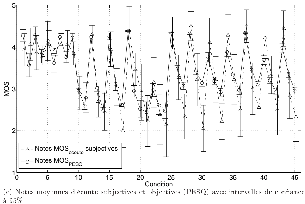
Figure 5.6 : Performances de PESQ - Signaux de conversation
