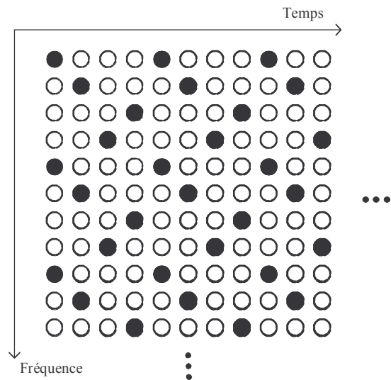
figure 24 : Canal lent
