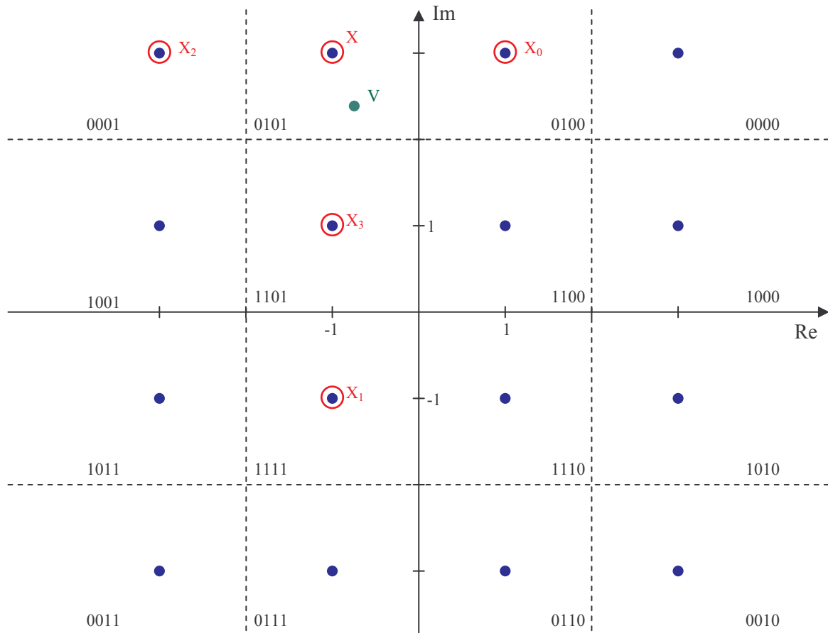
figure 45 : Constellation 16-QAM
