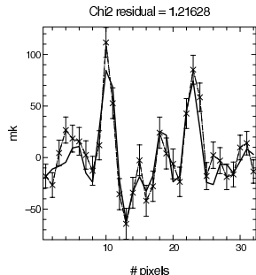
Fig. 4. Example of fringe-fitting by the carrying waves in the 3-telescope case. The DC-corrected interferogram is plotted (dashed line) with the error bars. The result of the fit is overlotted (solid line).
