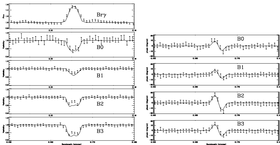
Fig. 16. \alpha Arae differential visibilities ( left ) and phases ( right ) across the B_{\gamma} line profiles for the B_0 , B_1 , B_2 , and B_3 baselines. The solid lines are the fits we obtain with SIMECA from the model 3 described in Sects. 4.3.2 and 6.6, whereas the AMBER/VLTI data are the points with error bars.
