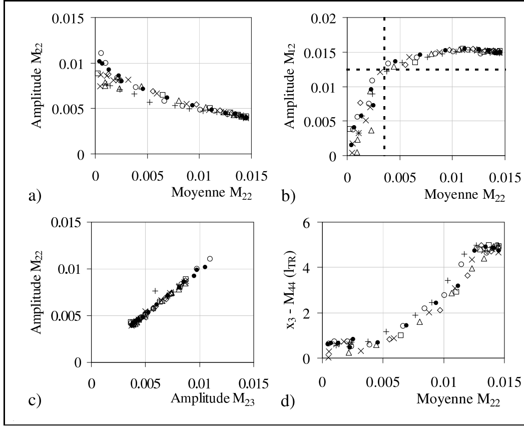
Fig. 7.10 Corrélations entre les informations issues de la matrice de Mueller. ( + m = 0, 75 , \circ m = 0, 90 , \bullet m = 1, 10 , \times m = 1, 20 , \triangle m = 1, 30 , \diamond m = 1, 50 , \square m = 1, 80 )
