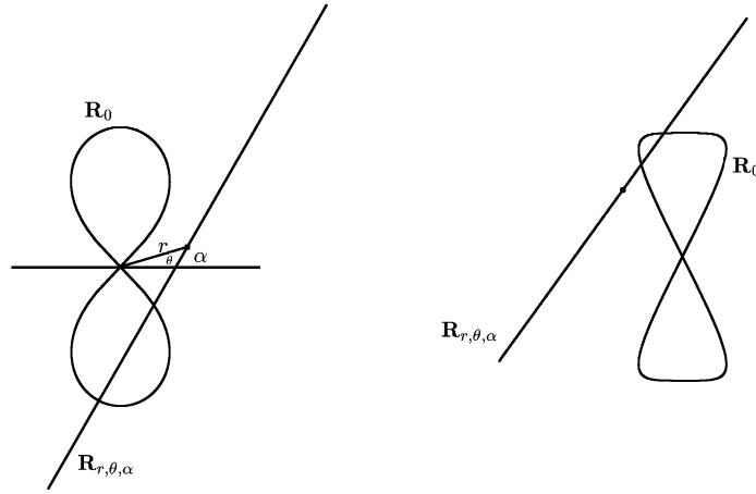
Fig. 2. \mathbf{R}_{r,\theta,\alpha} ; lateral view (right) and top view (left). The distinguished point is an intersection of the infinite \mathbf{R} -circle with the surface of centers of \mathbf{R}_0 .
