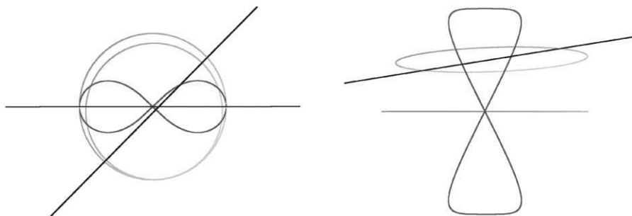
Fig. 6. Deformed configuration; lateral view (right) and top view (left) with invariant \mathbf{C} -circles.
