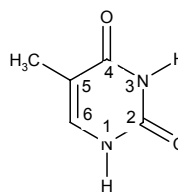
Thymine
