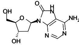
8-oxo-7,8-dihydro-2'-désoxyadénosine (8-oxodAdo)
