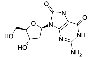
8-oxo-7,8-dihydro-2'-désoxyguanosine (8-oxodGuo)
