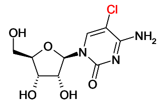
5-chloroCytidine (5-ClCyd)
