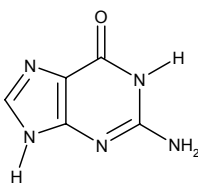
Guanine
