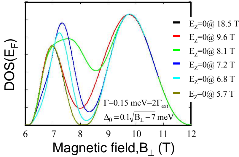
Figure 4.32: Angle dependence of the calculated \text{DOS}_{\text{ext}}(E_F) in the vicinity of \nu=3 considering \Delta_0 = f(B_{\perp}) at T=2\text{K} . The zero Zeeman energy ( g^*=0 ) is noted for each plot.
