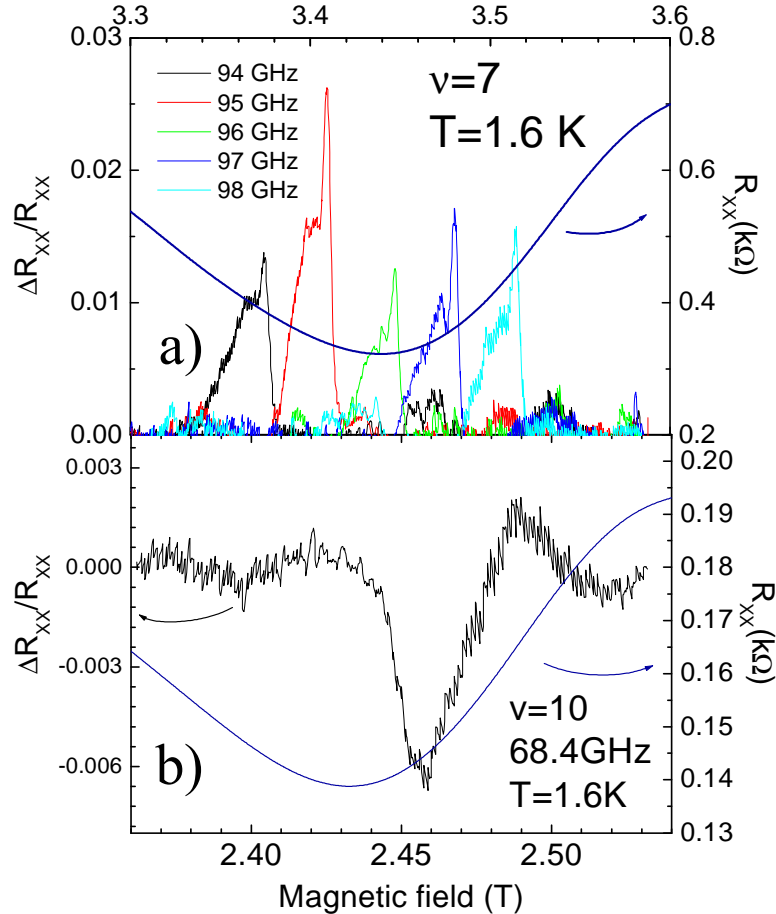
Figure 5.3: a) Relative change of the longitudinal resistance \Delta R_{xx}/R_{xx} (left axis) at T=1.6K for different microwave frequencies near to \nu=7 . The R_{xx} in absence of microwaves (blue line) is presented for comparison with the resonant position. b) Relative change of the longitudinal resistance \Delta R_{xx}/R_{xx} (left axis) at T=1.6K for 68.4GHz microwave illumination near to \nu=10 .
