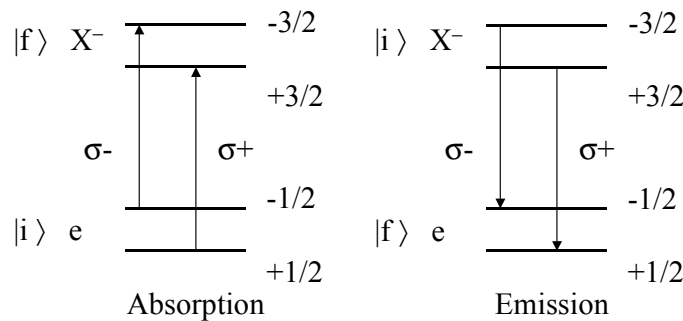
Figure 1.14. Schema of the allowed optical transitions, absorption (left) and emission (right) for e + h\nu \leftrightarrow X^- . The spin of h is the hole spin, the two electrons being spin-paired.
