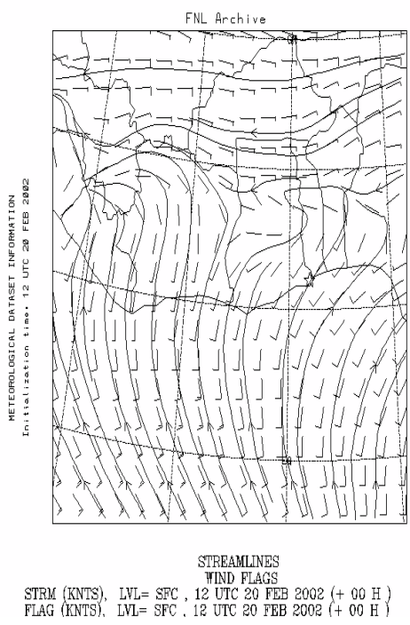
Figure 5.1. (e)-(h) Typical wind streamlines over Ghana during the Harmattan period.
