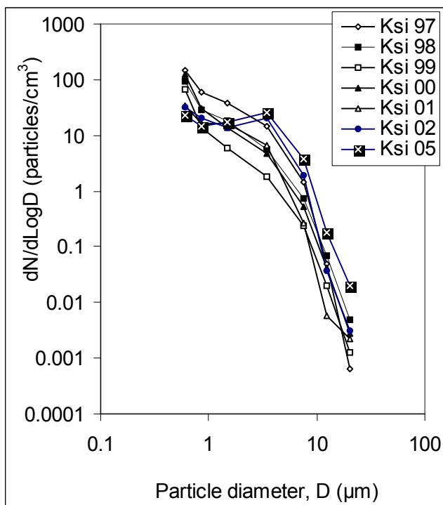
Figure 5.12. Particle number distribution in Kumasi during the selected Harmattan periods: 1997-2005.
