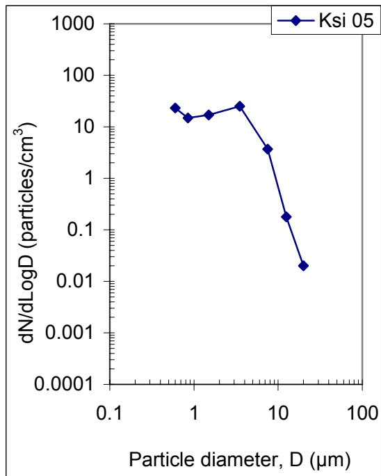
Figure 5.11. (g) Typical particle number distributions at Kumasi.
