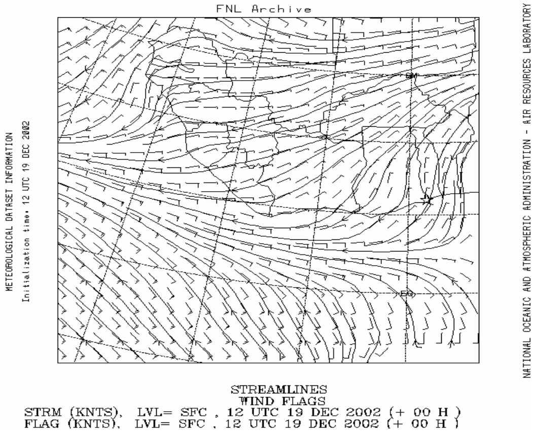
Figure 4.1. Sample chart of winds streamlines on 19 th December, 2002, over West Africa, showing the northeast and southwest streamlines meeting around latitude 2.6° N south Ghana.
