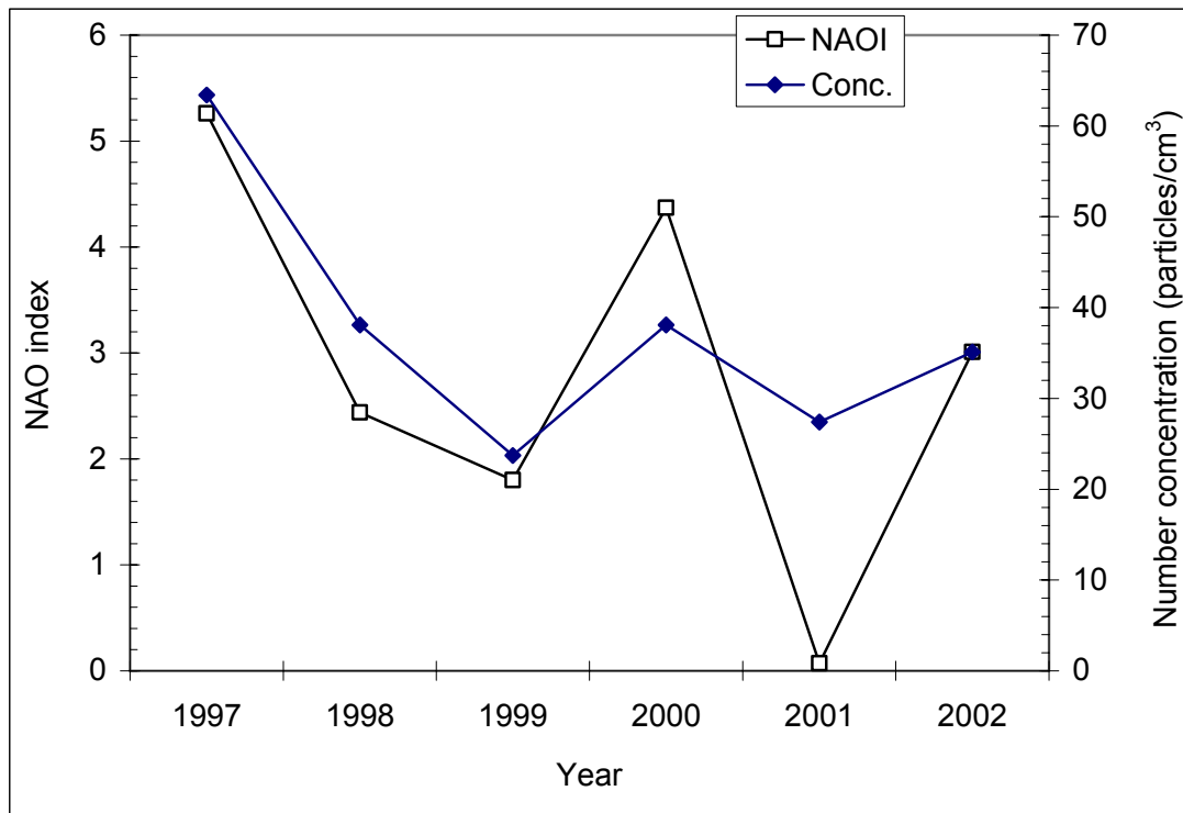
Figure 5.42. Comparison of NAO index in February and mean particle concentration at Kumasi in February: 1997-2002.
