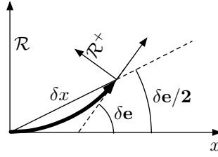
Figure 1.9: Odometry model with forward motion and Euler increments.
