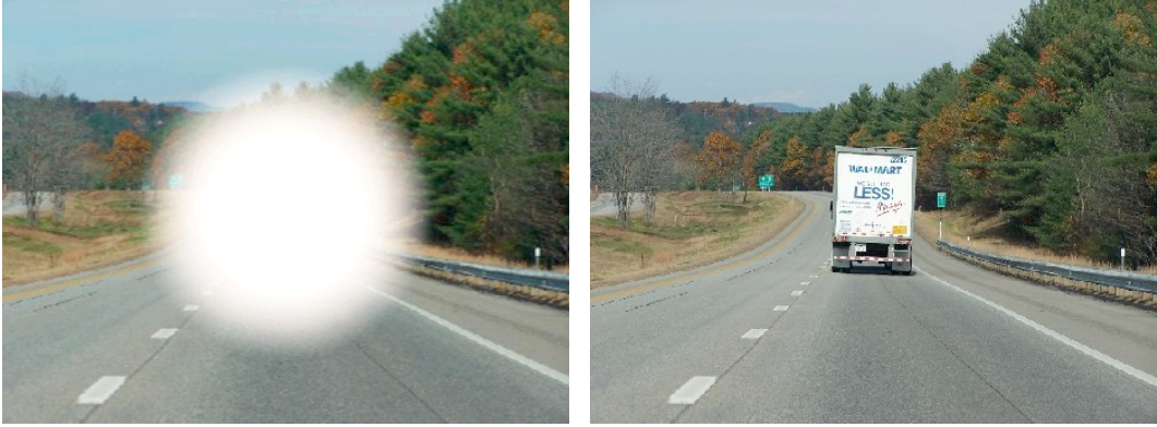
Figure 6.2: Delayed and undelayed operations. Frontal-blindness effect of delayed initialization ( left ) which leads to SLAM systems that only take into account fully observed landmarks, thus not those close to the motion axis. By considering also partially observed landmarks, an undelayed operation ( right ) is able to exploit all the available information.
