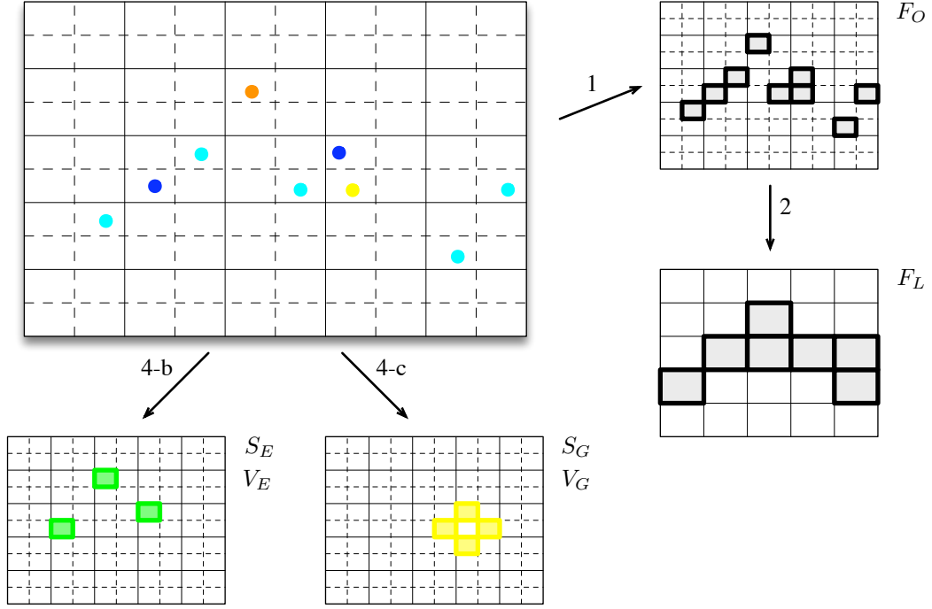
Figure 8.11: Priority-based Detection Selector algorithm -I-: Generation of matrices F_O , F_L , \{S_E, V_E\} and \{S_G, V_G\} from the set of projected 3D points in the image. Missed landmarks ( dark blue ) and missed objects ( orange ) activate the Event-driven DM cells ( green ); Matched objects ( yellow ) activate their four Object-growing DM neighbor cells. Matched landmarks are in pale blue . Existing features set cells in F_O which in turn set those in F_L (both in gray ). Arrow numbers refer to the corresponding step in the algorithm.
