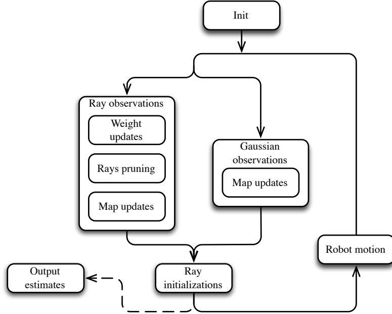
Figure 6.9: The FIS-SLAM algorithm.
