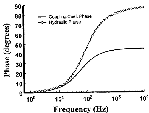
FIG. 3. Phase comparison of the frequency-dependent coupling coefficients and frequency-dependent hydraulics, where the phase is 0^\circ for both curves at 0 Hz.
