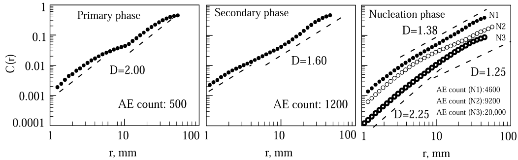
Fig. 9. Correlation integral function for the hypocenters in the HF sample against distance using logarithmic coordinates. The fractal dimensions estimated from the slope are also shown.
