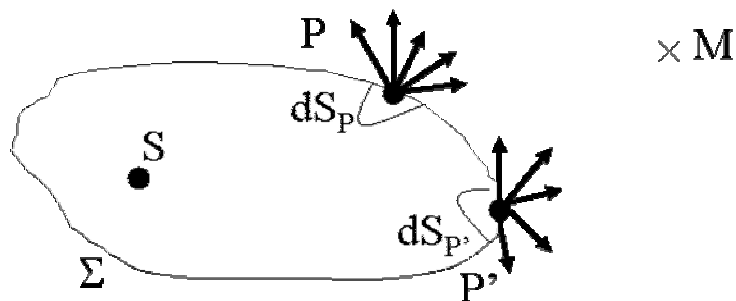
Figure A- I-2: Principe de Huygens-Fresnel
