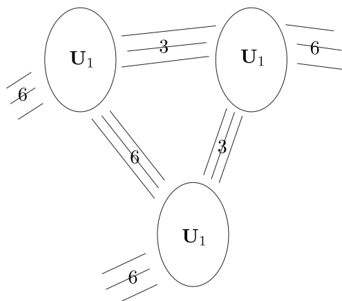
FIGURE 6. U_{\{1,3,6\}} .
