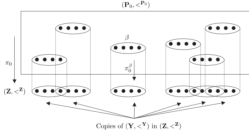
FIGURE 3. Construction of \mathbf{P}_0 .
