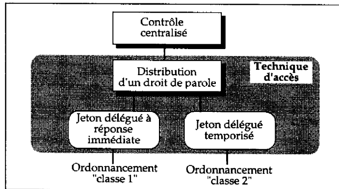
Figure 3.16: Le protocole IEC 65C
