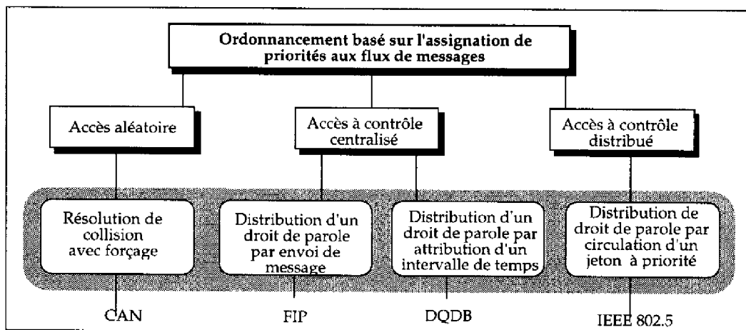
Figure 3.3: Les protocoles "classe 1" existants
