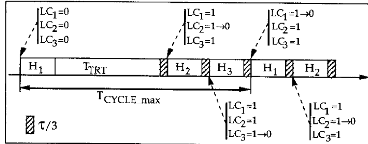
Figure 3.14 Diagramme temporel
