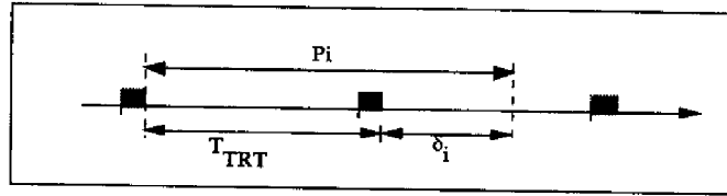
Figure 4.6: Relation entre P_i , \lfloor P_i/T_{TRT} \rfloor et T_{TRT}
