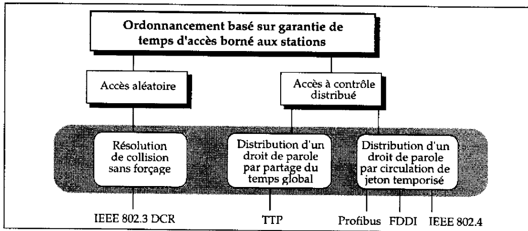
Figure 3.12: Les protocoles "classe 2" existants
