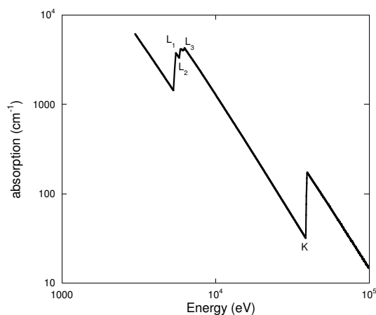
Figure 3.9: Absorption coefficient evidencing the discontinuities associated to K -, L_{1,2,3} -edges.
