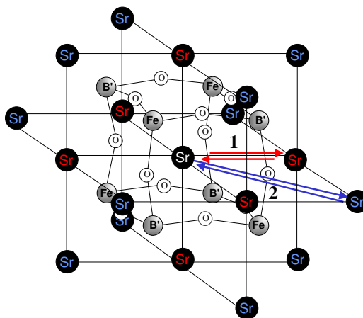
Figure 6.15: Representation of the first four coordination shells in the case of Sr absorber. 12-fold and 6-fold degenerate selected photoelectron paths are labeled 1 and 2 for the third and fourth shell respectively.
