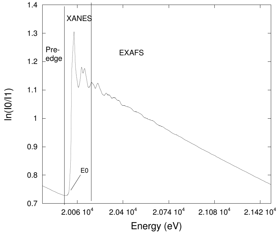
Figure 3.10: Absorption K-edge of the Mo atom ( E_0 = 20000 eV). Post-edge EXAFS oscillations are evident compared to the smooth pre-edge and far post-edge atomic background.
