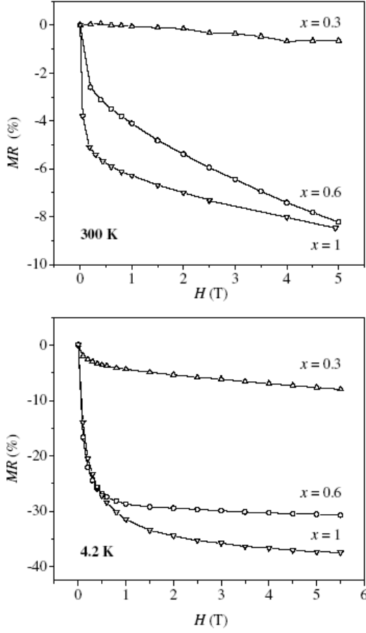
Figure 2.12: Percentage of magnetoresistance for x = 0.3, 0.6 and 1 at 300 K (upper panel) and 4.2 K (lower panel).
