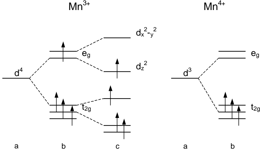
Figure 1.5: Left panel: a) 3d^4 five-fold degenerate \text{Mn}^{3+} electronic levels; b) 3d levels splitting due to the crystal field; c) Further splitting due to the JT effect. Right panel: a) 3d^3 \text{Mn}^{4+} levels; b) crystal field splitting of the 3d levels.
