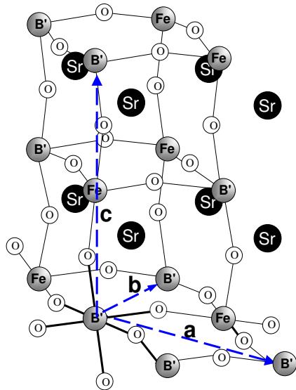
Figure 6.3: Double-perovskite cubic cell. The dashed arrows indicate the lattice vector a , b and c . Note that a = b \neq c for the tetragonal cell ( I4/m ) and a \neq b \neq c for the monoclinic cell ( P2_1/n ).
