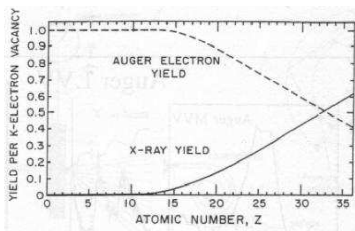
Figure 3.6: Calculated Auger electron and X-ray yields per K vacancy as a function of atomic number (Sieghahn et al.)
