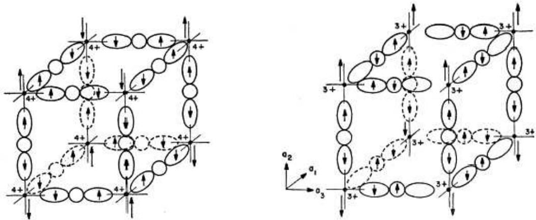
Figure 1.11: Magnetic lattice type G ( x = 1 ).
