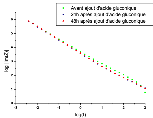
d- \log |Im(Z)| = f(\log(\text{fréquence}))
