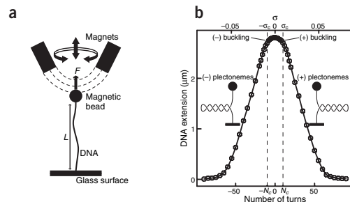
Figure 1 Stretching and supercoiling a single DNA molecule. (a) Experimental setup. A single DNA molecule is connected to a magnetic bead (1- \mu\text{m} diameter) and the interior of a square glass capillary. Magnets placed above the capillary stretch the molecule with a constant force F ; the resulting DNA extension, L , is measured in real-time by optically tracking the bead's position. Rotating the magnets introduces a controllable number of supercoils into the DNA molecule. (b) Extension of a supercoiled DNA molecule stretched with 0.3 pN. The molecule has its maximum extension when relaxed (0 added turns). Small numbers of added turns twist the DNA without substantially changing the extension. The molecule buckles after N_c \approx 10 turns have been added; given the measured 4.3 \mu\text{m} contour length, this corresponds to \sigma_c \approx 0.008 . Turns added beyond buckling form plectonemes that cause a linear decrease in extension with rotation with a typical slope m_p \approx 70 \text{ nm turn}^{-1} .
