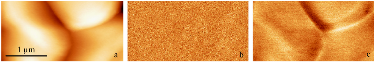
Fig. 3. Topography (a), CPD measured with a lift (b) CPD measured with a linear scan mode (c) of the same area of a sputtered Al layer. Peak to valley values are respectively 66 nm, around 8 meV (noise level) and 27 meV. To allow comparison, potential color scales are identical.
