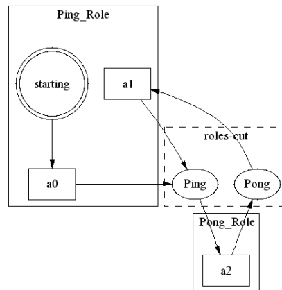
Figure 4.7: The roles and roles-cut of the 'ping-pong' coordination protocol.
