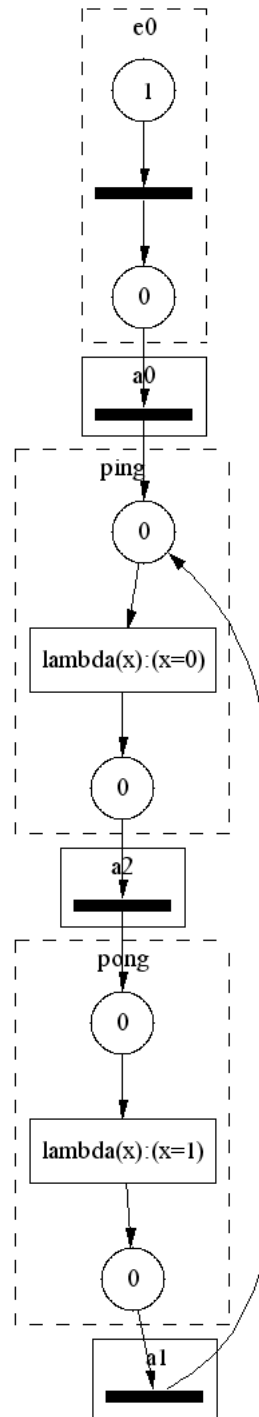
Figure 4.12: The QPN associated to the ping-pong coordination protocol.
