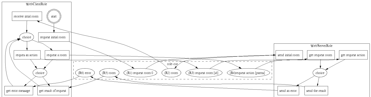
Figure 5.11: The coordination protocol of the WEBACTIVITY social task.
