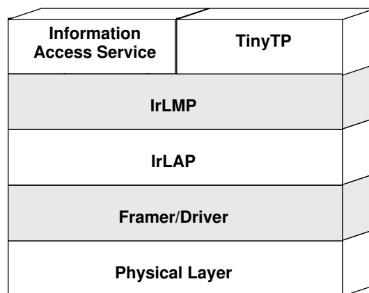
Figure F.3: The IrDA protocol stack [Knutson & Folsom, 1999].
