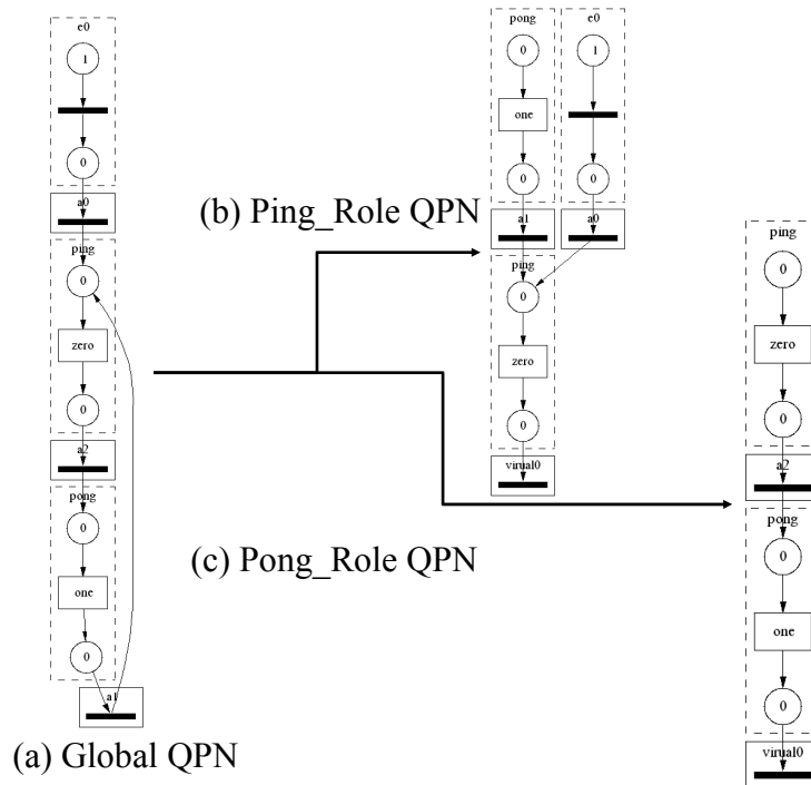
Figure 4.17: The QPN of the global coordination graph of Figure 4.16 and its decomposition on roles.
