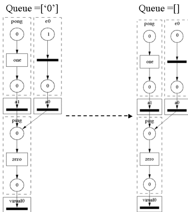
Figure 4.19: The initial and final state of the QPN associated to the 'PingRole' sub-coordination graph.
