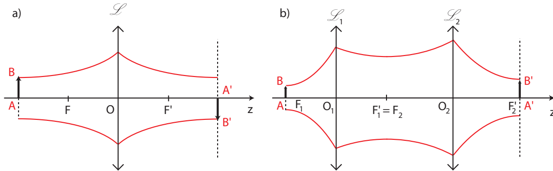
Figure 4.2: The two most simple imaging setups, a) "2f-2f" and b) "f 1 -f 1 -f 2 -f 2 " configurations. In both cases, object AB and image A'B' planes are situated at waists position, and the magnifying factor equals 1.
