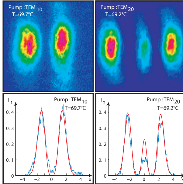
Figure 4.11: SH profiles generated in the crystal far field with \text{TEM}_{10} and \text{TEM}_{20} collimated pump modes, i.e. in the thin crystal approximation. The cross-section traces contain both the data and theory fits. Pump modes and optimal phase matching temperatures are reported on each inset.
