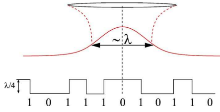
FIG. 2. (Color online) Example of a bit sequence on an optical disk. The spacing between the bits is smaller than the wavelength, the minimum waist of the incident laser beam being of the order of \lambda . A hole depth of \lambda/4 insures a \pi phase shift between fields reflected on a pit and a hole.
