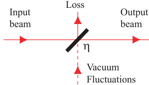
Figure 1.3: Modelisation of loss on a quantum state using a partially reflecting beam-splitter of transmission \eta . The noise properties of the output state are modified by the vacuum fluctuations entering via the empty port of the beam-splitter.
