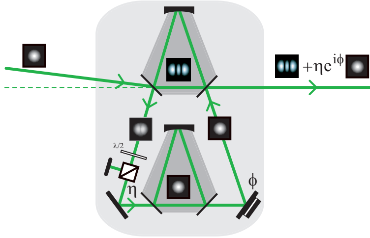
Figure 4.19: Proposition to generate an optimal pump mode for a TEM 10 operation of the OPA cavity with two ring cavities. An incident green TEM 00 mode is misaligned in order to couple into the TEM 20 component of the first ring cavity. The cavity is locked to the TEM 20 mode. The reflected field is then filtered with a second ring cavity in order to produce a pure TEM 00 mode. The amplitude ratio \eta and the relative phase \Phi can be varied using a variable attenuator and a piezoelectric device, respectively.
