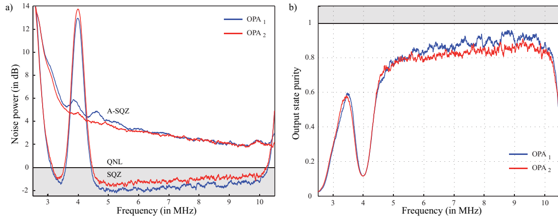
Figure 5.11: a) Squeezing and anti-squeezing spectra of \text{OPA}_1 (blue trace), and \text{OPA}_2 (red trace). The spectra have been back inferred from measurements using the whole setup, and have been corrected for electronic noise. b) Purity of the states generated at the output of \text{OPA}_1 (blue trace), and \text{OPA}_2 (red trace). Both curves have been corrected for losses after the output of the devices. Resolution and video bandwidth were set to 300 kHz and 300 Hz respectively.
