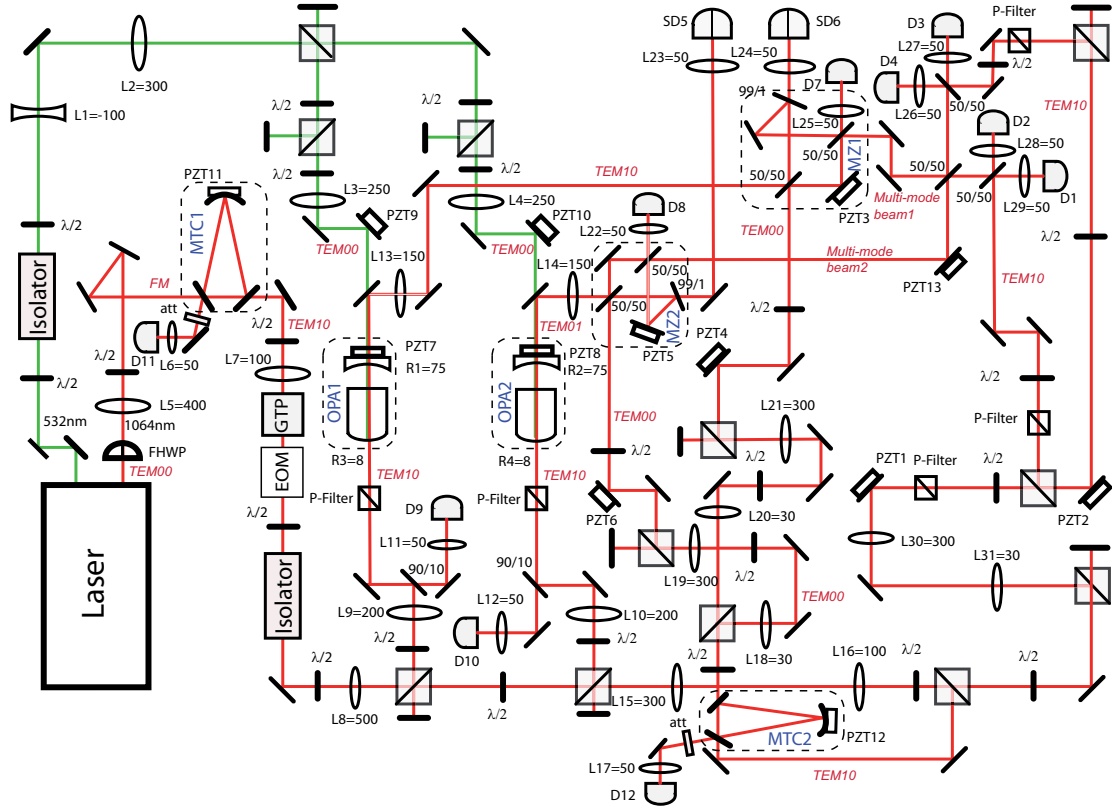
Figure 5.9: Experimental setup for spatial entanglement. D: detector, SD: split-detector, L: lens (focal length in mm), R: radius of curvature (in mm), FWHP: flipped mode half-waveplate, GTP: Glen-Thomson polarizer, EOM: electro-optic modulator, att: attenuator, P-Filter: polarization filter, PZT: piezoelectric device.
