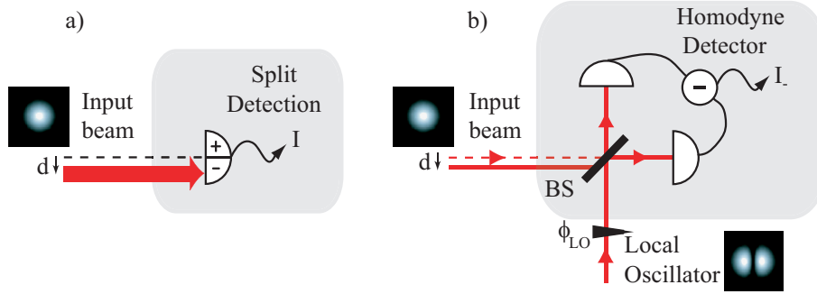
Figure 3.5: Beam displacement detection devices. a) split-detection. b) TEM 10 homodyne detection.
