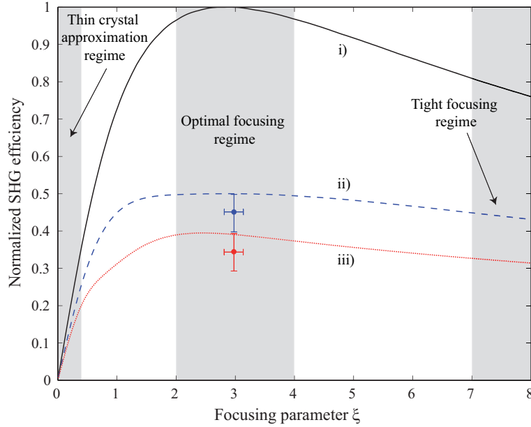
Figure 4.12: SHG efficiency as a function of the focusing parameter \xi , in optimal phase matching conditions, for i) TEM_{00} , ii) TEM_{10} and iii) TEM_{20} pump modes. All curves are normalized to the best conversion efficiency obtained for the TEM_{00} case. We have represented the three most relevant regimes to our analysis : 'thin crystal approximation regime' corresponding to collimated beams, 'optimal focusing regime', and 'tight focusing regime'. Two experimental points corresponding to the measurements presented in Table 4.2 are represented in the optimal focusing region.
