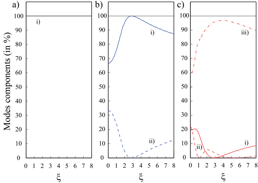
Figure 4.13: Modal decomposition of the SH field as a function of the focusing parameter \xi , in optimal phase matching conditions, for a) \text{TEM}_{00} , b) \text{TEM}_{10} and c) \text{TEM}_{20} pump modes. Mode components are represented in percentage of the overall power. In all insets, trace i) corresponds to a \text{TEM}_{00} SH component, whereas traces ii) and iii) respectively refer to \text{TEM}_{20} and \text{TEM}_{40} SH components.
