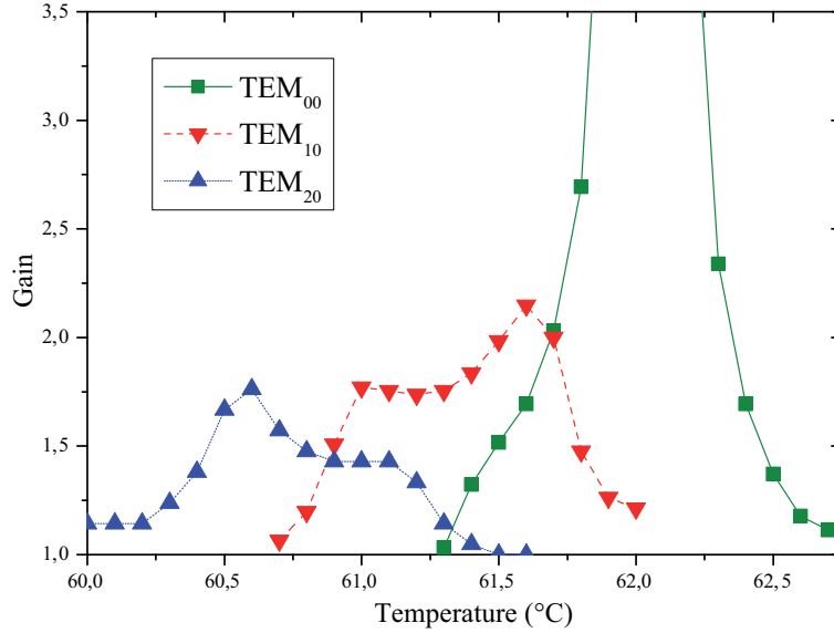
Figure 4.21: Classical gain factor as a function of the crystal temperature for OPA operation with a TEM 00 , a TEM 10 and a TEM 20 signal modes. The optimal phase-matching temperature are 62.1°C, 61.6°C and 60.6°C for the TEM 00 , TEM 10 and TEM 20 H-G modes, respectively.
