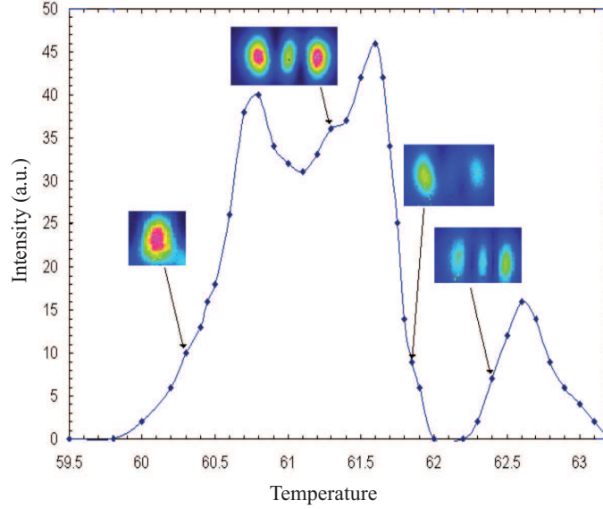
Figure 4.22: SHG operation of the OPA cavity. The intensity of the SH beam is plotted as a function of the crystal temperature, when the seed beam is a TEM_{10} infrared mode. Some profiles of the generated SH beams are also presented. Phase-matching curve for the nonlinear crystal and different SHG TEM modes as a function of temperature.
