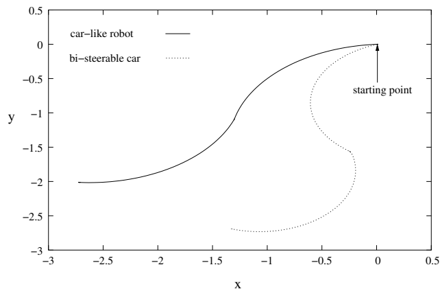
Figure II.6: Bi-steerable car's maneuverability characteristics: Simulated traces of the point (x_R, y_R) using models (II.2) and (II.8). These traces are obtained when applying the same typical commands, for a parallel parking maneuver, to a conventional car-like robot (top track) and to a BiS-car for which the rear-front coupling relation is a constant of proportionality held to 0.7 (bottom track).
