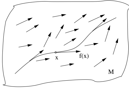
Figure A-2: Vector field and integral curve on a manifold.
