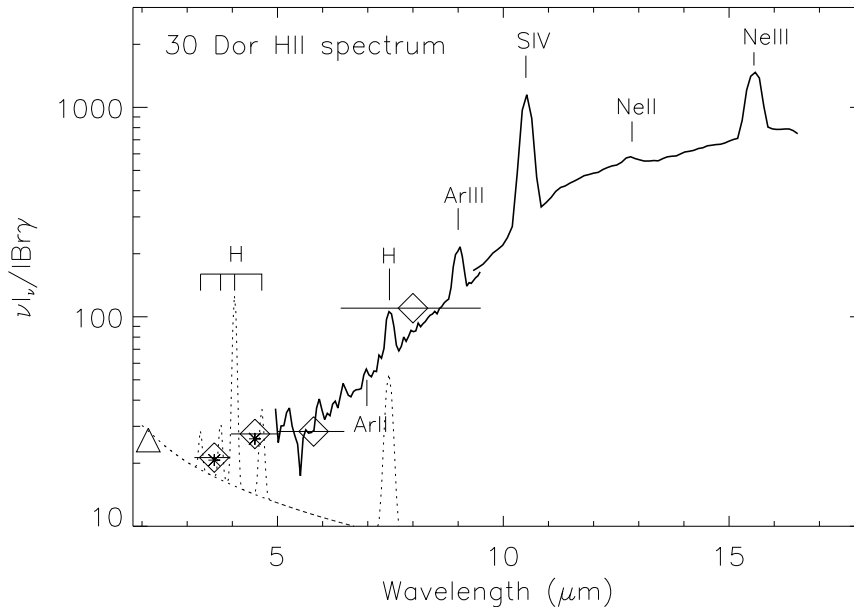
Fig. 8. Mid-IR spectrum from the 30 Doradus HII gas (Section 4). The spectrum is normalized per unit Br \gamma line intensity. The diamonds represent the fluxes derived from the IRAC images, the triangle that from the near IR image at 2.14 \mu\text{m} . The dotted line represents the continuum (free-free+free-bound) and the main H-recombination lines emission from the ionized gas (Section 6). The stars represent the gas emission in the 3.6 and 4.5 \mu\text{m} IRAC filters.
