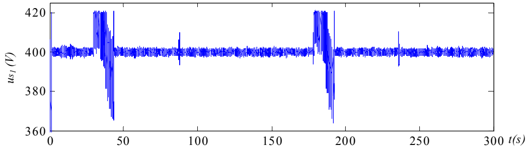
Fig. 2.40b: Tension du bus continu DC.
