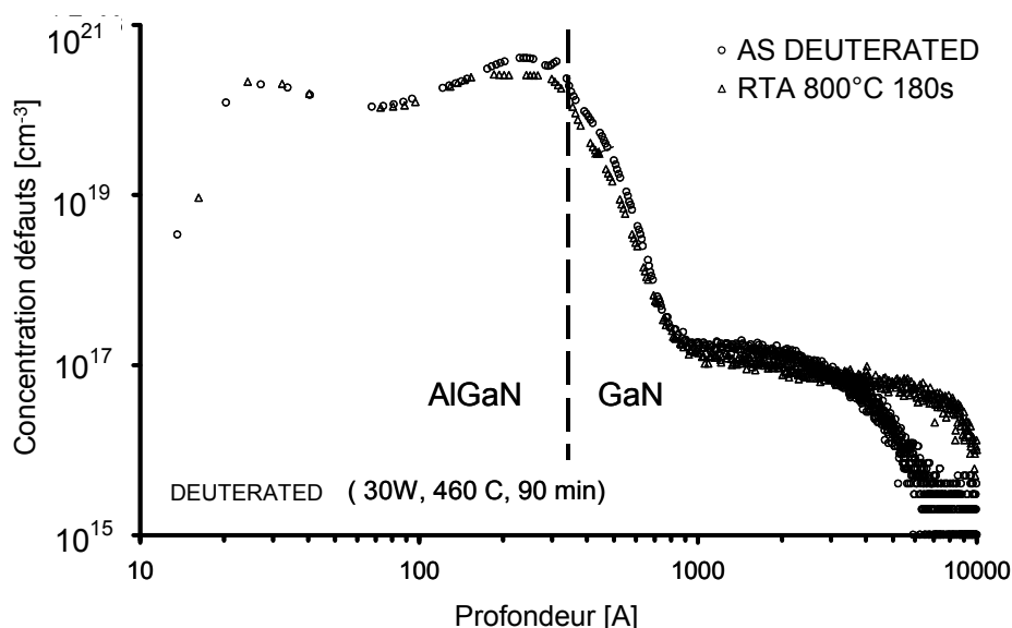
Fig 2.22 Etude SIMS LPSC Meudon, J. Mimila-Arroyo, J. Chevallier [10] ; contrat ANDRO
