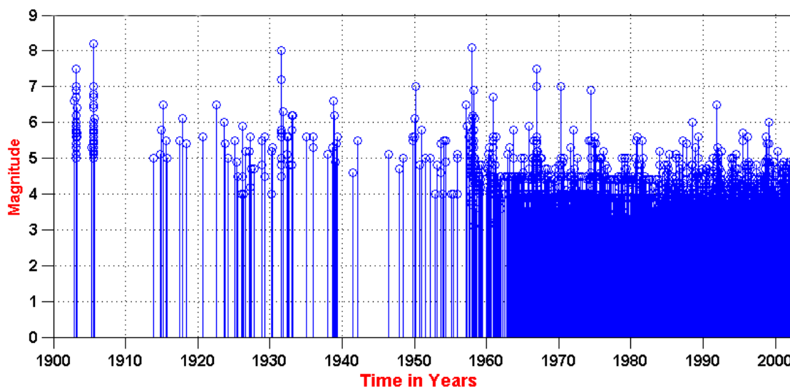
Figure II.12: Distribution of the maximum magnitude observed in Mongolia function of time.
