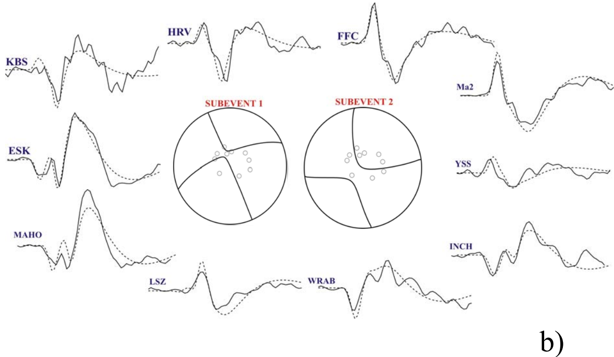
Figure V.22. Telesismic waveform modelling result of first large aftershock of the Chuya earthquake. The fitting between observed (solid line) and synthetic (dashed lines) P (a) and SH (b) waveforms are improved. Stations are ordered clockwise by azimuth.
