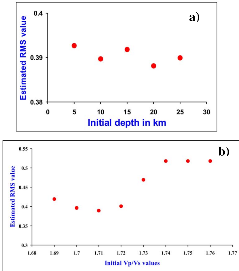
Figure IV.21. Variation of the global RMS with (a) starting depth and (b) Vp/Vs ratio.
