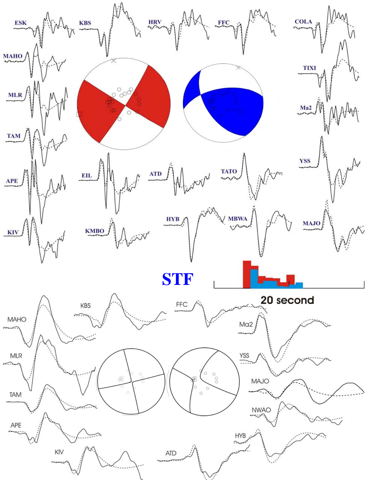
Figure V.29. The observed (solid line) and the best-fitted synthetic (dashed line) P and SH seismograms for the model bilateral propagating line source. This model has been chosen to be the best model on the fitting of observed and synthetic P wave forms criteria for the last
