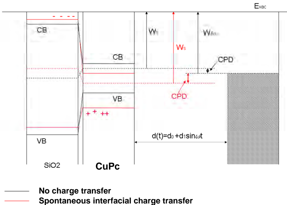
Figure 4.12b Energy level diagram of CuPc|glass with gold electrode at a distance of d(t) with or without spontaneous interfacial charge transfer
