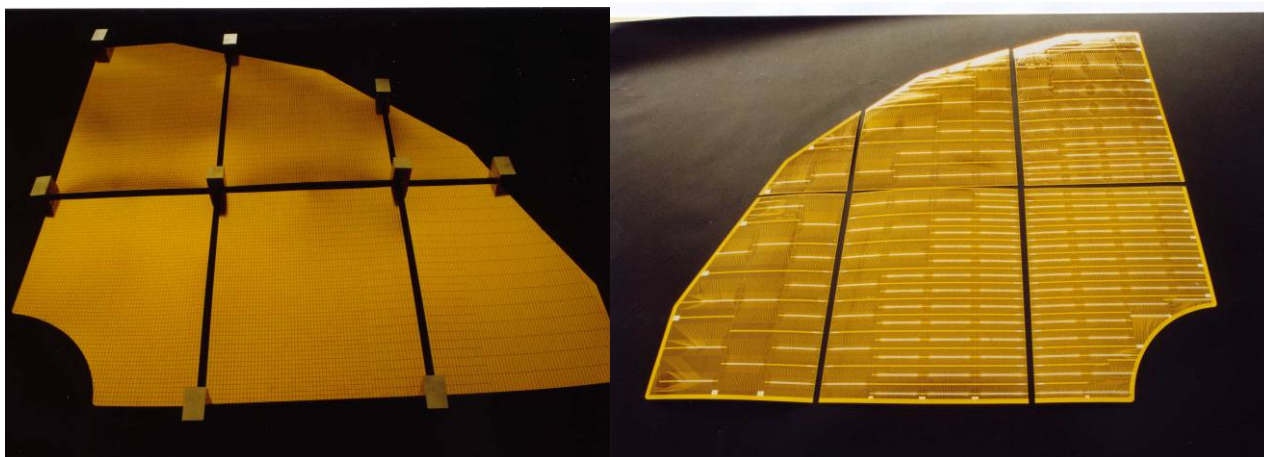
Figure 62 : Photograph of the 6 individual PCB's used to build up the full cathode plane. The left hand side shows the view of the pads and the right hand side shows the backside with the readout circuits. The variable pad and connector densities are visible.
