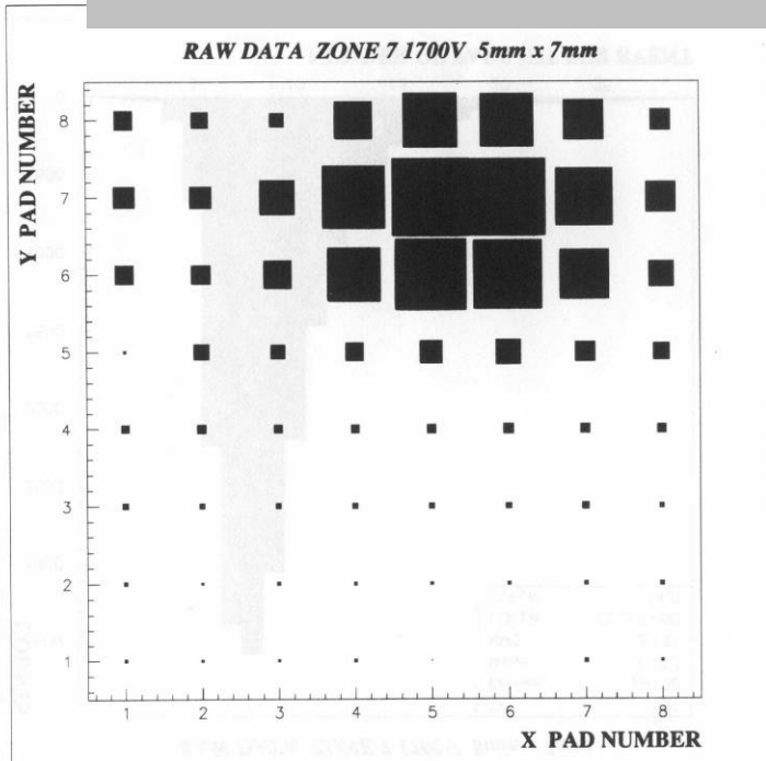
A first level reconstruction algorithm maps the gassiplex channel numbers to digital (X,Y) impact points. The beam impact area is obvious on the left hand figure. The four most frequently hit pads are analyzed. Their amplitudes are shown on the right hand side image. Apart from the general form of the distributions, the number of saturated pads indicates whether the electronics dynamical range is sufficient for the particular detector gain setting.
