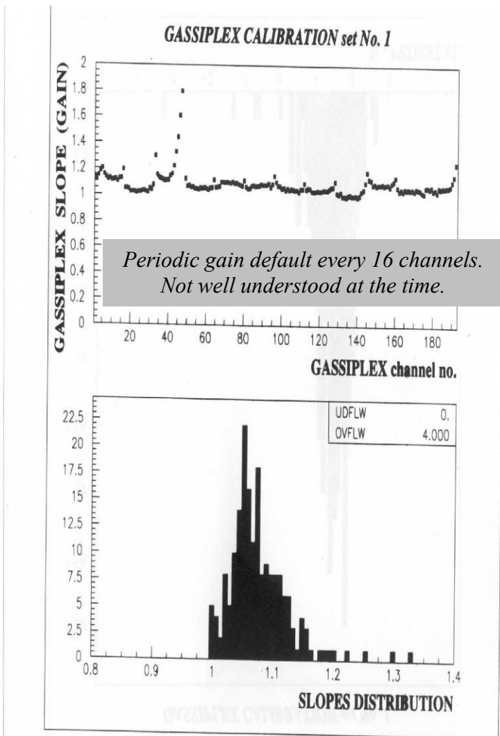
Calibration curves for 192 channels comprised of the straight line fit results.
