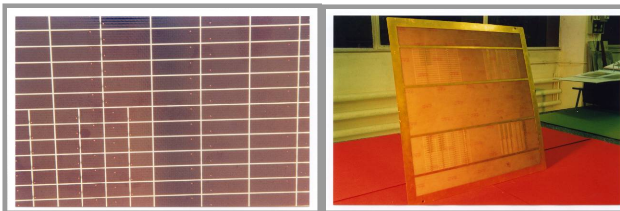
Figure 40 : Photographs of the copper pad plane (LHS), the feed through holes on each pad are visible. This image shows the junction between two pad sizes. The other image (RHS) shows the back side of the pad plane engraved on the PCB. The four distinct pad areas are visible.
