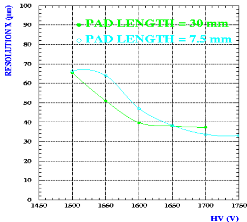
Resolutions for two different pad lengths as a function of HV.
