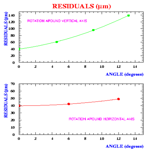
Resolutions for varying angles on 30 mm long strips and with a 2.5 mm wire pitch at 1600 V. More details can be found in reference [35], pp.93-95.
