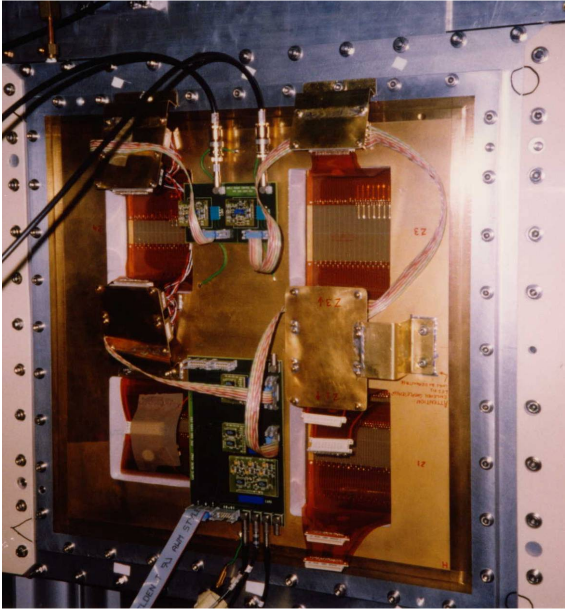
Figure 43 : ALICE1 in situ at the PS in CERN. The multiple scattering contribution was minimized by placing the electronics on the side of the active surfaces. The effective thickness was estimated to be 1.2% of a radiation length.
