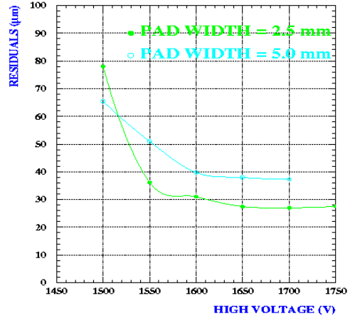
Resolutions for two different pad widths as a function of HV.
