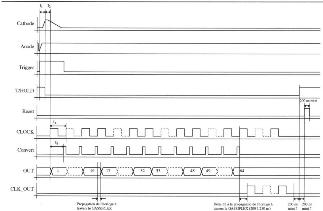
Figure 32 : Timing sequence for the sequential ADC readout with t_1 = 700 ns, t_2 = 170 ns, t_3 = 260 ns (not shown on image), t_4 = 520 ns, and t_5 = 260 ns
