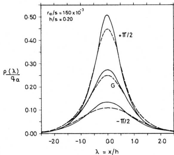
Fig. 3. Comparison of empirical distributions, G , with exact distributions; \rho_1 (full curves) and \rho_2 (broken curves). The exact distributions were calculated at a time 1.0 \mu s , for avalanche angular positions \alpha = +\pi/2 and -\pi/2 , with rms angular spread \sigma = 40^\circ , and for s = 3.0 \text{ mm} , V_a = 0.8 \text{ kV} and \mu = 1.9 \text{ cm}^2/V_s . The total cathode charges, relative to the net anode charge, are -0.71 ( \rho_1 and \rho_2 ) for +\pi/2 , 0.29 for -\pi/2 and necessarily 0.5 for G . The empirical distributions represent K_3 = 0.70 for \rho_1 and 1.0 for \rho_2 .
