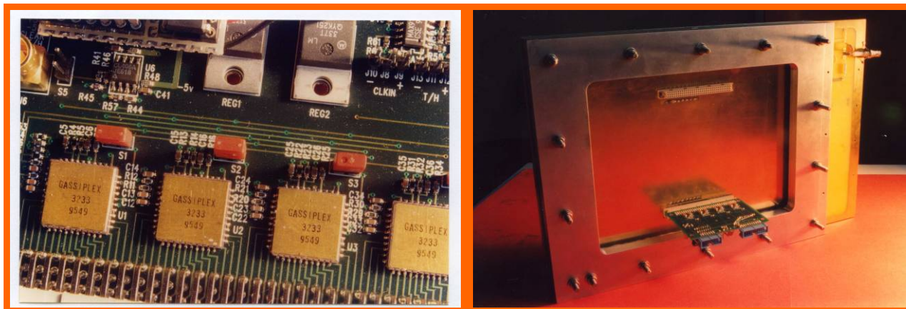
Figure 31 : On the left hand side (LHS), a close-up of the GASSIPLEX chips, each chip capable of measuring the charge amplitude on 16 individual pads. The chips are read in sequence through a common bus. On the right hand side (RHS), the first GASSIPLEX card at the IPN, Orsay, mounted on the detector.
