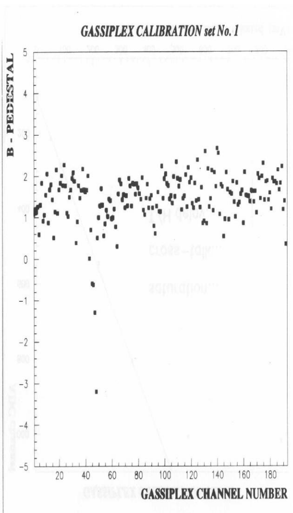
Calibration curves for 192 channels comprised of the straight line fit results.
