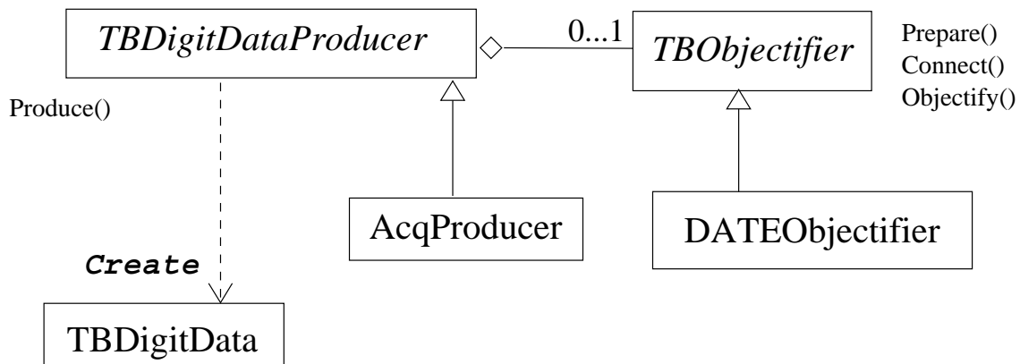
Figure 86 : UML diagram showing the general architecture of the data stream objectification.
