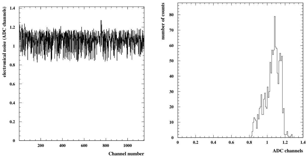
Figure 74 : The experimental electronic noise per channel is shown on the left, and the overall distribution on the right.
