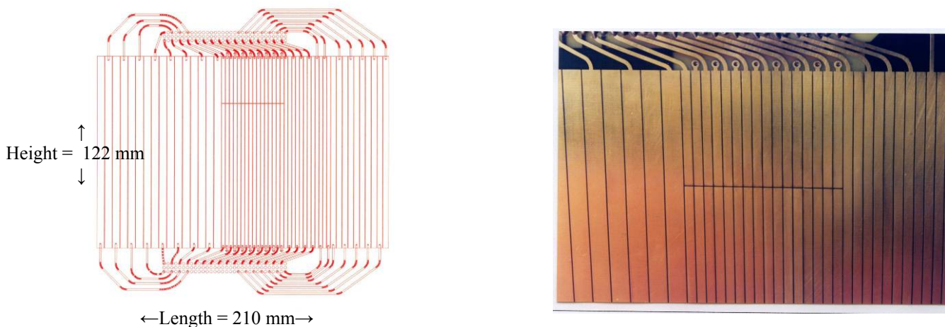
Figure 28 : The LHS shows the design of the cathode plane layout with the different pad sizes and the readout strategy. The RHS shows the upper central area of the finished object.
