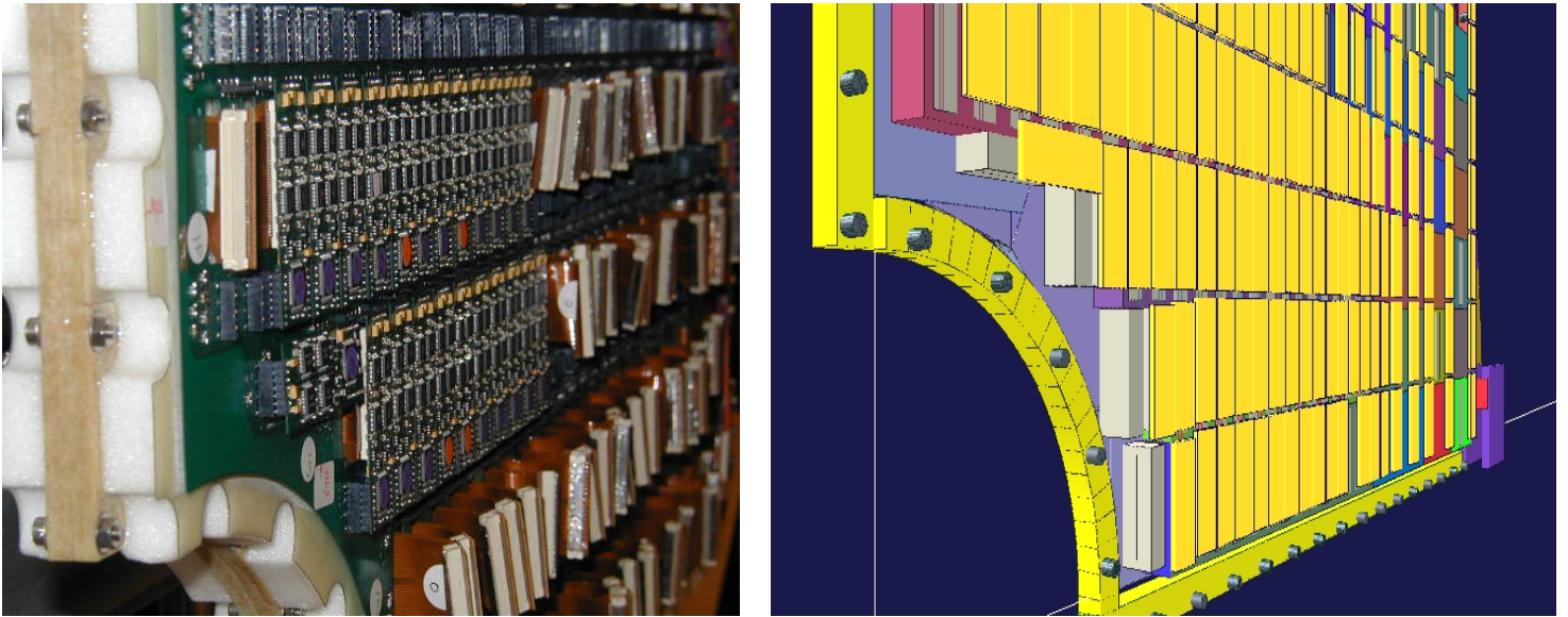
Figure 95 : On the LHS, photograph of the inner arch of QUADRANT0, and on the RHS the equivalent simulated object.
