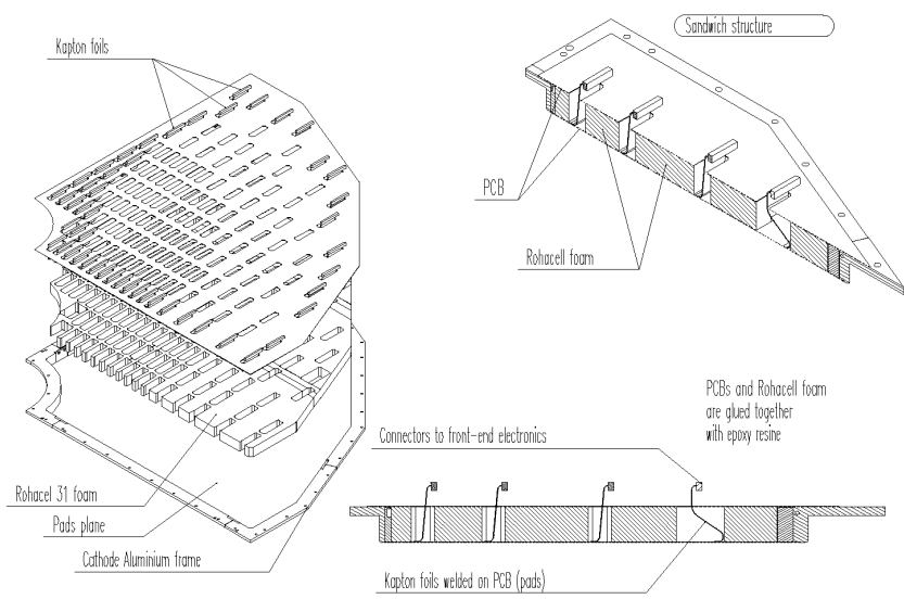
Figure 57: Cathode mechanical structure. The rigidity of the design is ensured mainly by the Rohacel foam which constitutes the heart of the structure.
