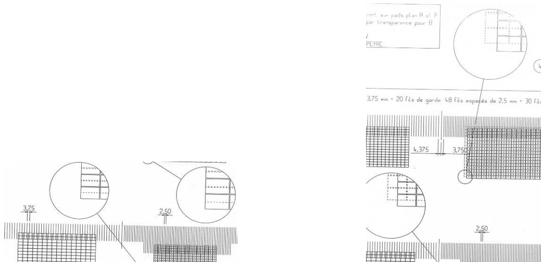
Figure 84: The two images show the relative pad positions through a transparent view of the cathode planes. The magnified part of the images shows the plane A pads drawn as full lines, with respect to the Plane B pads which are drawn with dashed lines. On the LHS the pads are offset by a half-pad in one direction and on the RHS, with Plane A rotated through 180°, the pads are offset by one half-pad in two directions. The wire grid can be seen in these images with the two different wire spacings at 3.25 mm and 2.5 mm.
