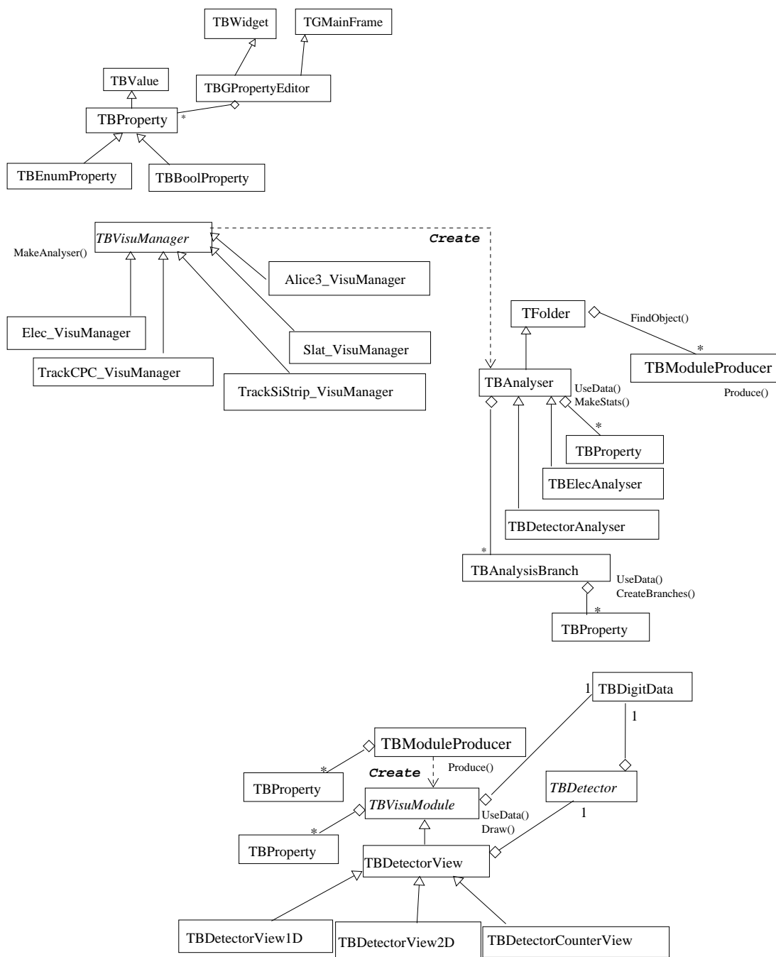
Figure 8: Analysis and graphical viewing classes. See section 3.4 for more details.
