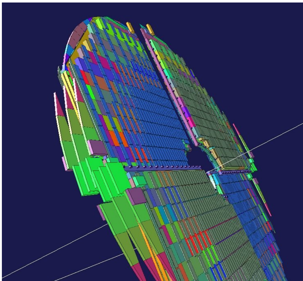
Figure 93 : General view of the station 1 detectors, complete with support frames, electronics cards and true layout.
