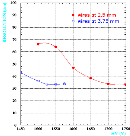
Resolutions for the two different wire pitches as a function of HV.
