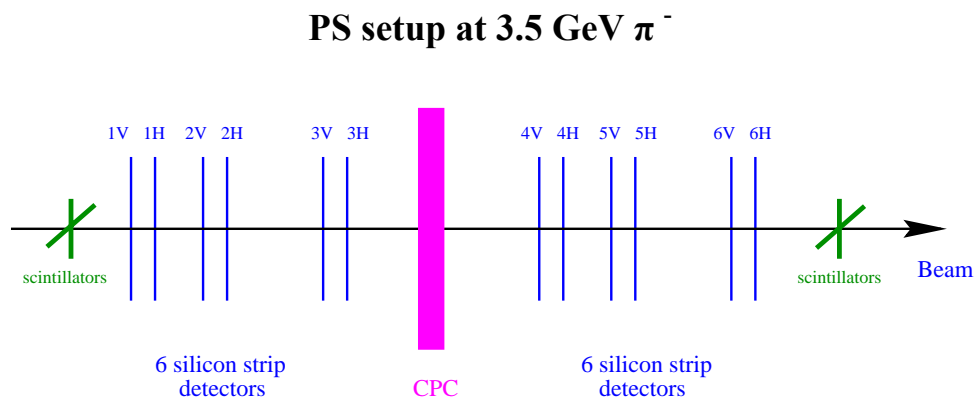
Figure 42 : Principle of the PS test beam layout: the trigger for the 3.5 GeV pions is given by a four fold coincidence between the two crossed scintillators and collimates the selected trajectories over 1 cm 2 . The CPC, along with 6 horizontal silicon strip and 6 vertical silicon strip detectors were readout with the DATEv2 acquisition system.
