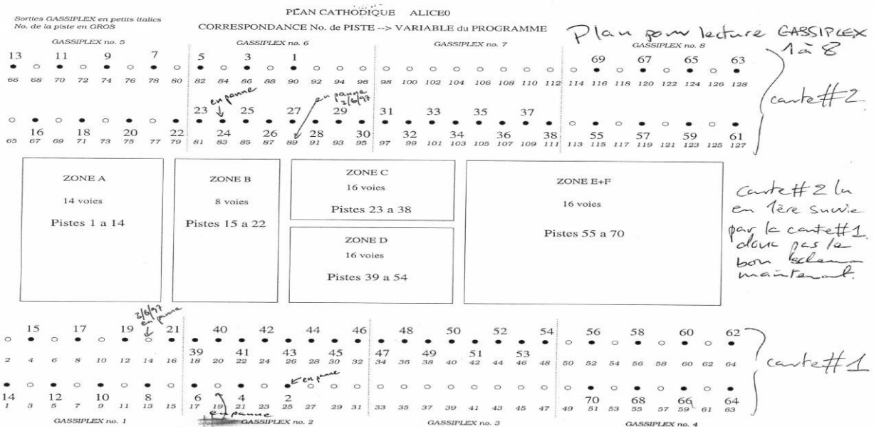
Figure 33 : View of the detector zones, A-F, and the associate readout mappings. Large numbers are the strip ID numbers and small numbers are the GASSIPLEX pin attributions.
