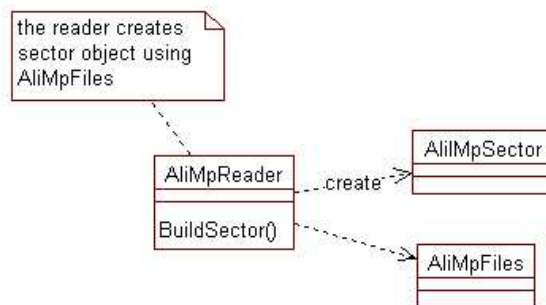
Figure 9: Sector reader class diagram.
