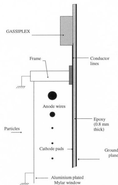
Figure 27 : Side view showing the general scheme for the detector layout.
