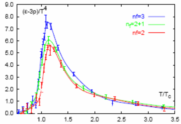
Figure 2 : The ‘interaction measure’, \Delta = (\epsilon - 3P)/T^4 versus T.
