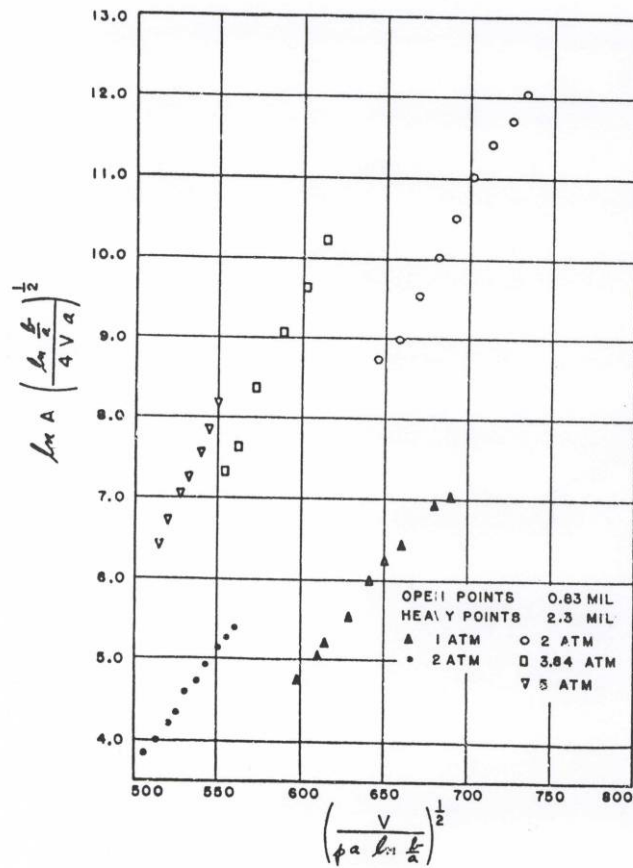
Figure 13 Test of Curran-Craggs Equation with Experimental Gas Amplification Factors for CH 4
