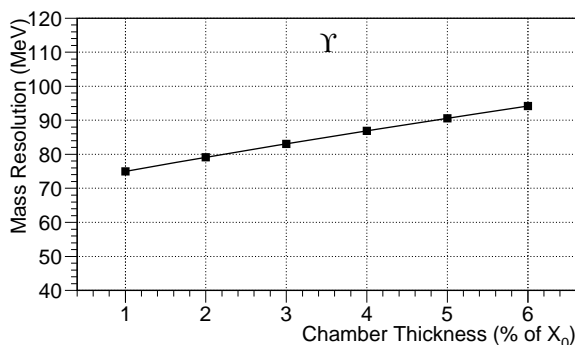
Figure 21: Expected mass resolution versus chamber thickness for the Y particle.
