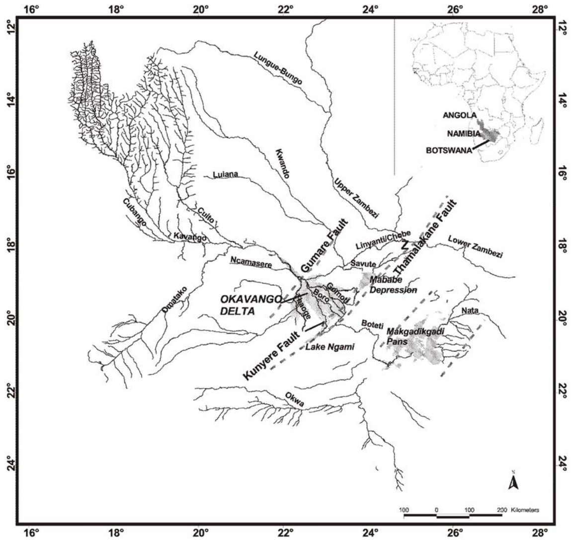
Figure VII 1. Okavango Delta in NW Botswana showing Lake Ngami to the south-west.
