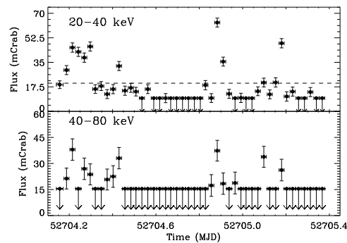
Fig. 2. The 20–40 keV ( top ) and 40–80 keV ( bottom ) ISGRI lightcurves. Each symbol represents a science window. The 3-sigma upper limits are denoted with an arrow. The dashed line in the upper panel indicates the 20 mCrab level.
