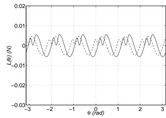
(f) Spatial unsteady lift, a\Theta = 0.5 rad
