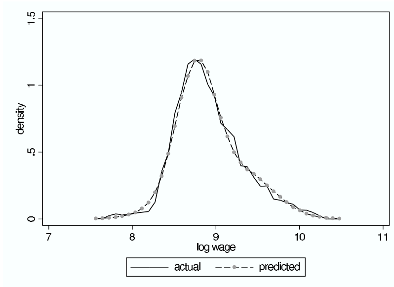
Figure 1.3: Cross-sectional earnings fit for K_1 = 3
