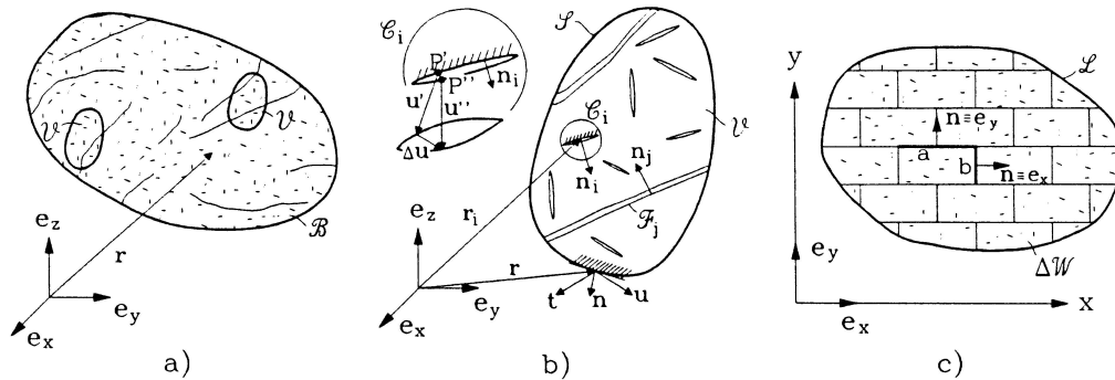
FIG. 1. (a) Small portions \mathcal{V} of a body \mathcal{B} containing microcracks and parts of large flaws; (b) displacement jumps at microcracks and flaws; (c) portion \Delta \mathcal{W} of a masonry wall.
