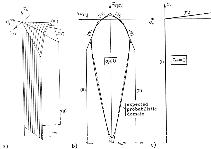
FIG. 6. Piecewise linear limiting surface of local possible equilibrium for a/b = 0.5 and \mu = 0.5 : (a) in the space of the stress state components \sigma_x, \sigma_y, \tau_{xy} ; (b) on a plane \sigma_y = \text{constant} ; (c) on the plane \tau_{xy} = 0 .
