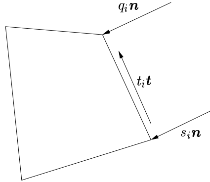
FIGURE 3.1 – Discretisation des efforts aux interfaces.
