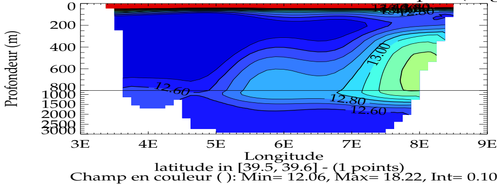
Section SAMM, date: 1977-1998, champ: T (degC)
