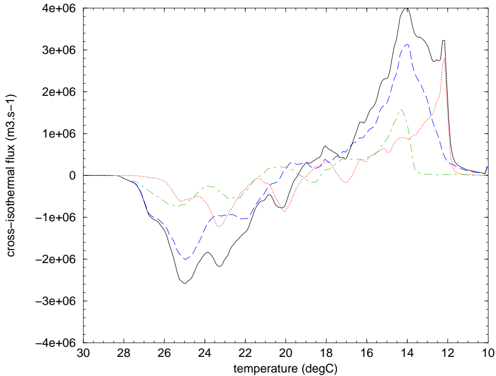
FIG. C.7 – Water mass transformations in \text{m}^3/\text{s} due to the surface flux, averaged over the whole period (1970-1998) for the OPAMED8 simulation : the whole Mediterranean Sea (solid line), the western part (dotted line), the eastern part (dashed line) and the Levantine basin (dotted-dashed line). The limit between East and West is at 13^\circ \text{E} and the western limit of the Levantine basin is at 25.5^\circ \text{E} . These curves allow the comparison with the study of Tziperman and Speer (1994).
