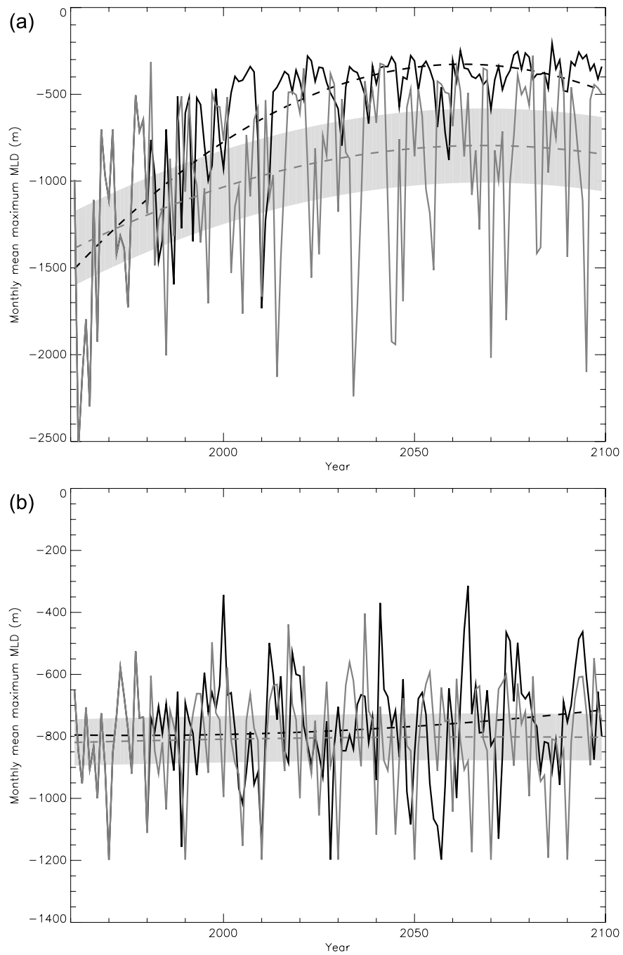
Fig. 8: Maximum depth reached by the monthly mean mixed layer depth (1 point per year - in meters) (a) for the Levantine Basin, (b) for the Adriatic Sea, (c) for the Gulf of Lions area, and (d) for the Aegean Sea. In grey, the control run (MC) and in black, the scenario (MS). A range corresponding to a 95% confidence level has been added for the fitted curve of MC
