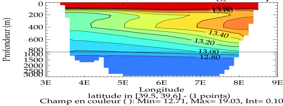
Section MEDATLAS-II, date: Climatology, champ: T (degC)
