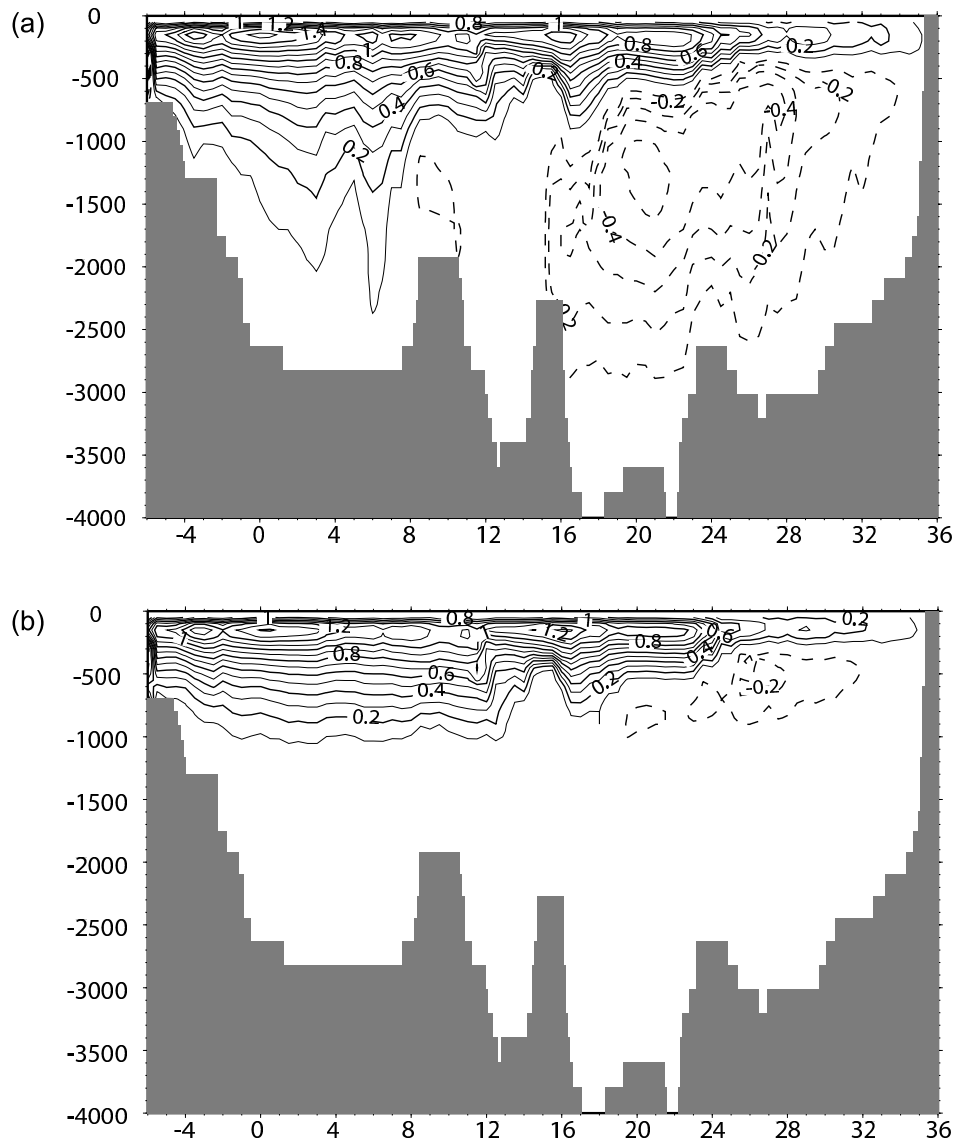
Fig 11: Vertical sections averaged over the 2070-2099 period for global Mediterranean Zonal Overturning stream Function (a) for the control run, and (b) for the scenario. The same calculation has been done for the Adriatic Meridional Overturning stream Function covering the Adriatic Sea plus the northern part of the Ionian Sea limited to 37°N (c) for the control run, and (d) for the scenario. The western Mediterranean Meridional Overturning stream Function limited to 38°N has also been computed (e) for the control run, and (f) for the scenario
