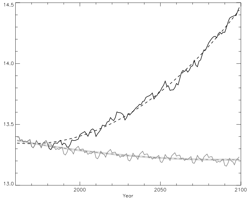
Fig. 5: As for fig. 2, but for the 3D averaged temperature of the Mediterranean Sea expressed in °C
