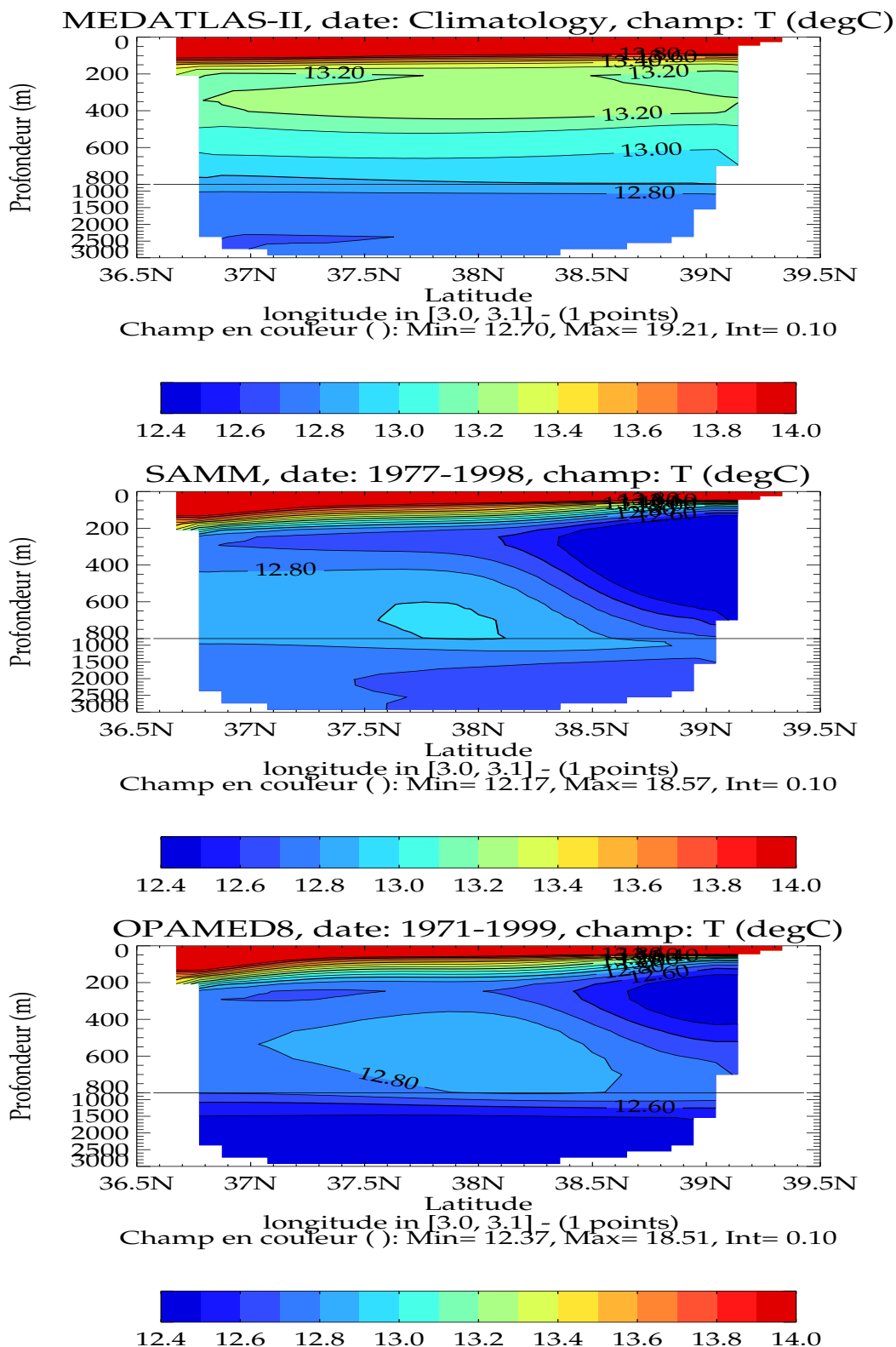
FIG. C.14 – Potential temperature vertical section for the Alboran Sea ( 3^{\circ}E ). This section corresponds to the section S1 in figure C.8. Top : MEDATLAS-II (climatology), Middle : SAMM (1977-1998), Bottom : OPAMED8 (1971-1999).
