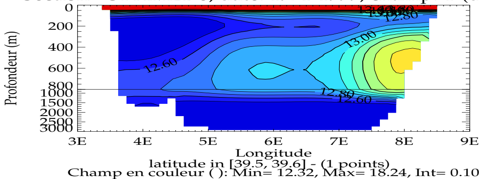
Section OPAMED8, date: 1971-1999, champ: T (degC)
