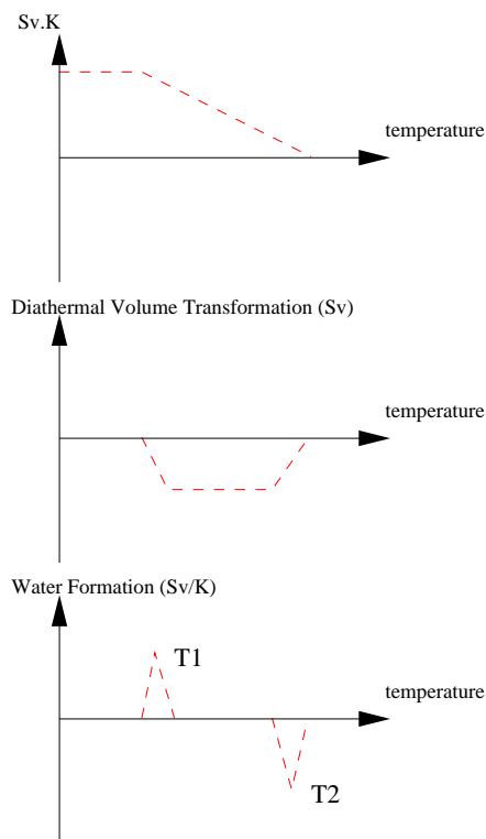
FIG. C.5 – Schematic of the diagnostic results of exchanging a cold water mass T2 for a warm water mass T1 ( X -axis inverted from high temperature to low temperature). At the top, integral of the transformation; in the middle, transformation and at the bottom, water mass formation ( 1 Sv = 10^6 m^3/s ).
