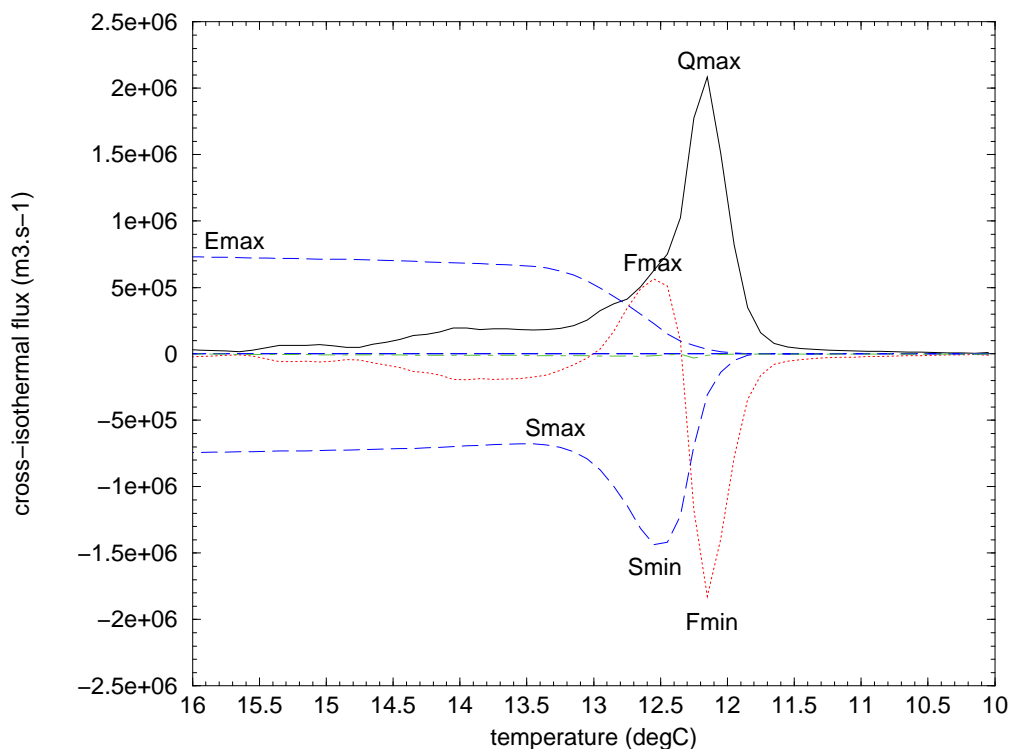
FIG. C.9 – Water mass transformations in m^3/s for the WMDW formation area (North-West of the Mediterranean Sea - see figure C.6), averaged over the whole period for the OM8-ARP simulation. Surface flux in solid line, mixing term in dotted line, advective term in dashed line (the southern border is negative and the eastern one is positive) and volume change term in dotted-dashed line.
