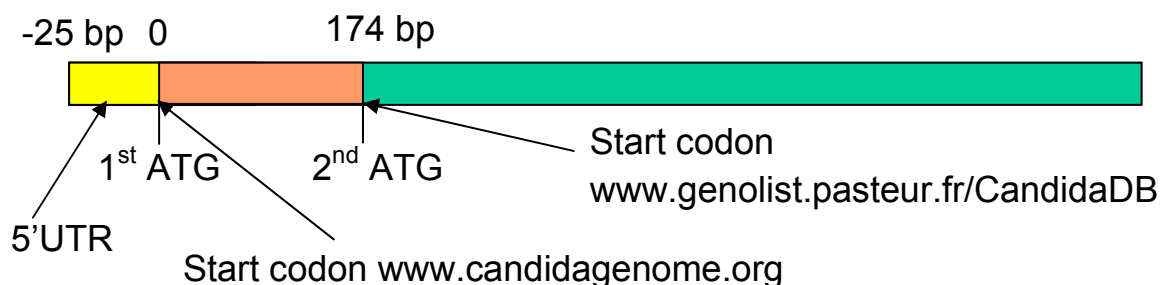
Figure 21: Analysis of the RIM101 transcript revealed that both possible start codons are transcribed with a 25 bp UTR sequence
