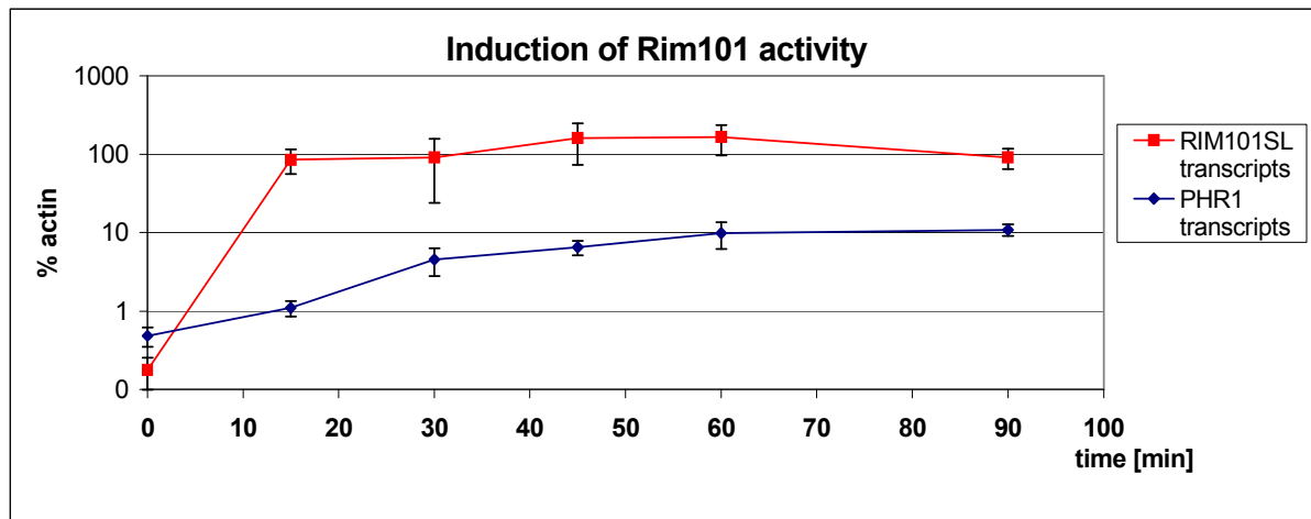
Figure 20: a) Validation of inducible Rim101 activity of strain FB8 on SC pH10 plates under MET3-inducing conditions in the Rim101SL strain (absence of methionine and cysteine) and under repressing conditions (presence of methionine and cysteine). Growth is compared to rim101 -/- disruption strain DAY25 and to reference strain DAY185 b) Real time PCR transcript quantification for RIM101SL and the Rim101 -induced gene PHR1 at 0, 15, 30, 45, 60 and 90 min growth in SC medium without Met/Cys
