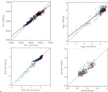
Fig. 3: Comparison to reference values compiled from the literature.
