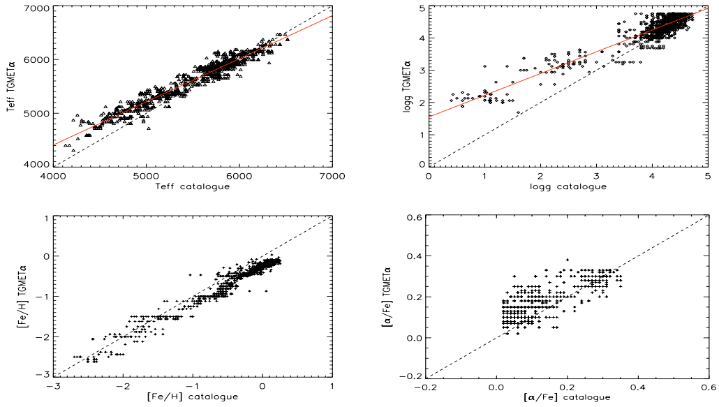
Fig. 10. Results at R=10000 for Teff, logg, [Fe/H] and [α/Fe] provided by TGMET \alpha vs literature values.
