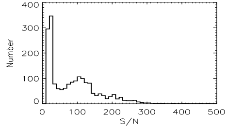
Fig. 8. Histogram of the S/N of our reference sample of 1874 spectra.
