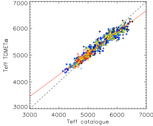
Fig. 3. Teff from TGMET \alpha vs Teff determined by each authors. “Plus” : Soubiran & Girard (2005); “triangles”: Ramírez & Meléndez (2005); “squares”: Blackwell & Lynas-Gray (1998); “circles”: Di Benedetto (1998); “diamonds”: Mishenina et al. (2006).
