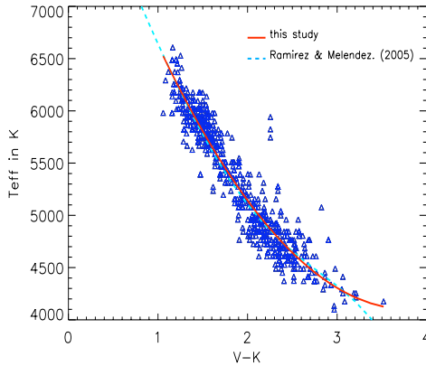
Fig. 4. Corrected Teff from TGMET \alpha vs V-K, fitted with a degree 2 polynomial. The relation for dwarf stars derived by Ramírez & Meléndez (2005) is shown by a dashed line.
