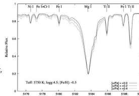
Fig. 1: A part of a synthetic spectrum.
