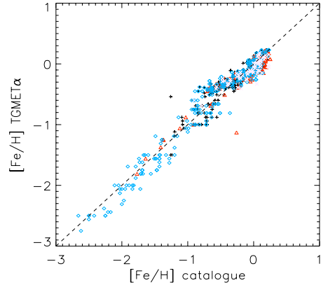
Fig. 5. [Fe/H] from TGMET \alpha vs [Fe/H] from the literature. Authors are marked with different symbols, “Plus”: Soubiran & Girard (2005); “diamonds”: Mishenina et al. (2006); “crosses”: Heiter & Luck (2003); “triangles”: Valenti & Fischer (2005).
