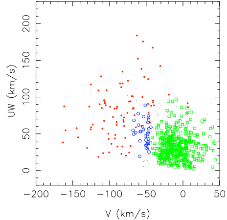
Fig. 9. As for Fig. 8, but in the Toomre diagram: UW = \sqrt{U^2 + W^2} km s ^{-1} .
