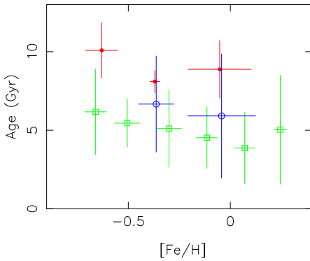
Fig. 12. Age vs. [\text{Fe}/\text{H}] for stars having well-defined ages. As in Figs. 8 and 9, the different symbols indicate thin disk, thick disk and Hercules stars.
