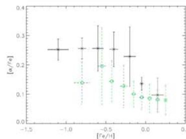
Fig. 4: [\alpha/\text{Fe}] vs [\text{Fe}/\text{H}] per bin of metallicity.
