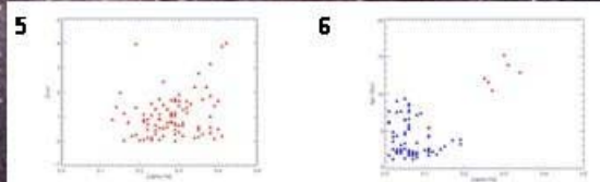
Fig.5 : Z_{\text{max}} vs [\alpha/\text{Fe}] for the thick disk stars.
