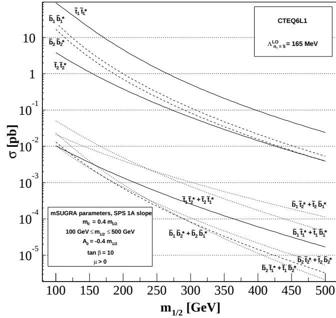
Figure 5.7: Production cross sections for top (full), bottom (dashed), and mixed top and bottom squarks (dotted) at the Tevatron (top figure) and at the LHC (bottom figure) as a function of the common fermion mass m_{1/2} in the mSUGRA model line SPS 1a [45].
