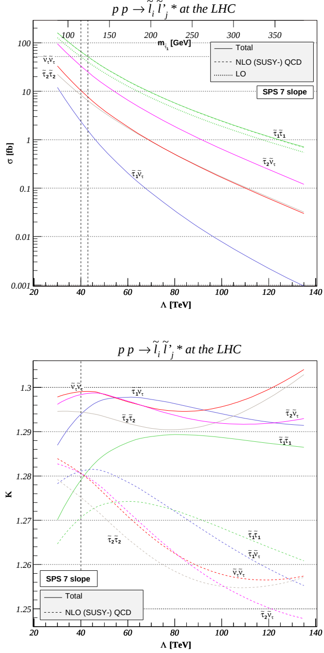
Figure 4.13: Total cross sections (top) and K -factors as defined in Eq. (4.68) (bottom) for third-generation slepton pair and slepton-sneutrino associated production at the LHC along the model line attached to the SPS 7 benchmark point (vertical dashed line). We show the total NLL+NLO matched and the fixed-order NLO (SUSY-)QCD and LO QCD results.
