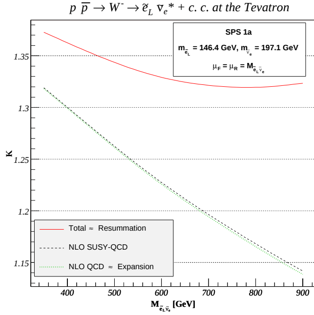
Figure 4.10: K -factors as defined in Eq. (4.67) for \tilde{e}_L pair (top) and associated \tilde{e}_L \tilde{\nu}_e^* production (bottom) at the Tevatron for the benchmark point SPS 1a. We show the total NLL+NLO matched result, which is almost identical to the purely resummed result at NLL, as well as the fixed-order NLO SUSY-QCD and QCD results. The latter practically coincides with the resummed result expanded up to NLO.
