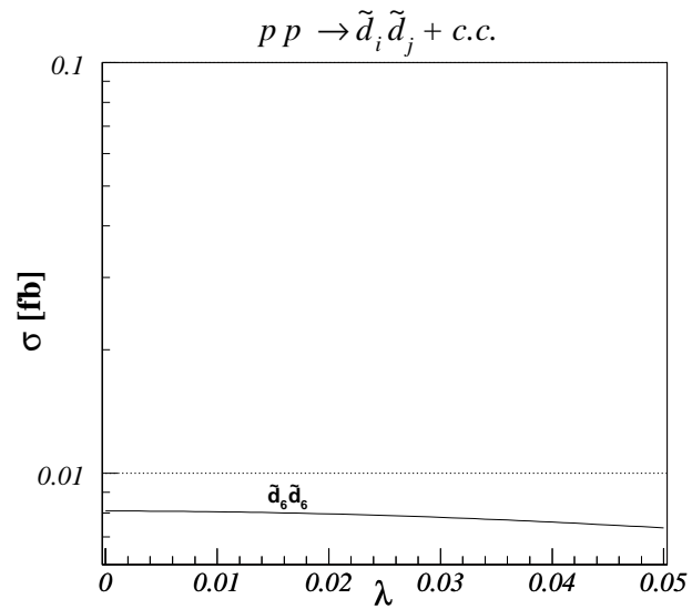
Figure 5.17: Same as Fig. 5.14 for our benchmark scenario D.
